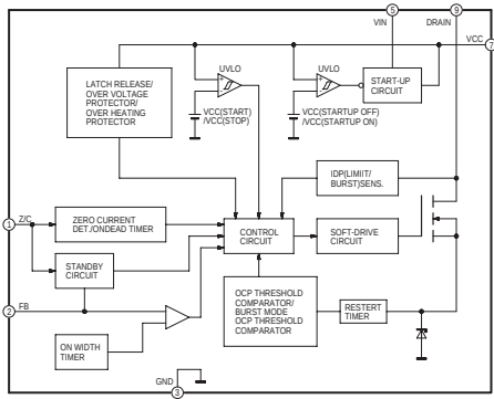
IC11201 SWITCHING IC IC-DETAIL BLOCK DIAGRAM
