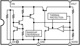
IC4801 AU +9V SWITCHING REG. IC-DETAIL BLOCK DIAGRAM
