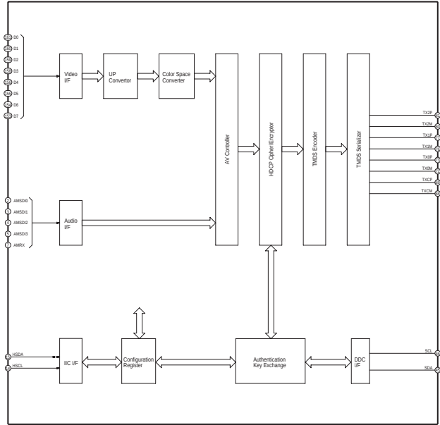
IC56103 HDMI TRANSMITTER IC-DETAIL BLOCK DIAGRAM
