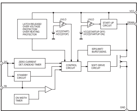
IC11301 SWITCHING IC IC-DETAIL BLOCK DIAGRAM
