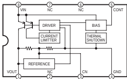
IC11720 F+ SWITCHING REGULATOR IC-DETAIL BLOCK DIAGRAM
