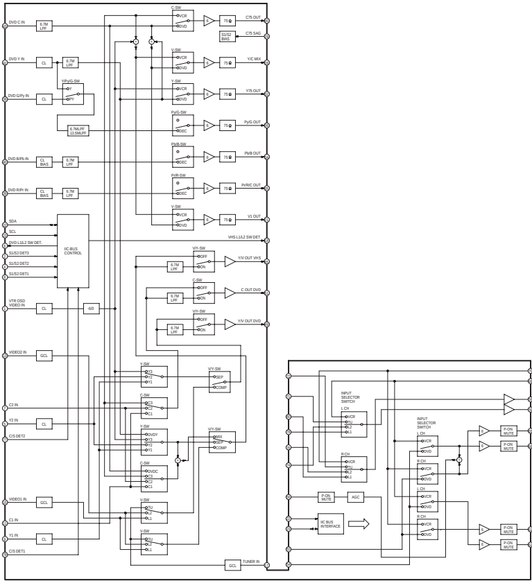
IC3701 VIDEO/AUDIO PROCESSOR IC-DETAIL BLOCK DIAGRAM
