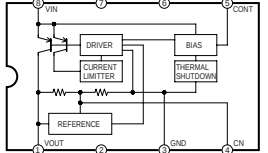
IC7402 TU +5V SWITCHING REG. IC-DETAIL BLOCK DIAGRAM
