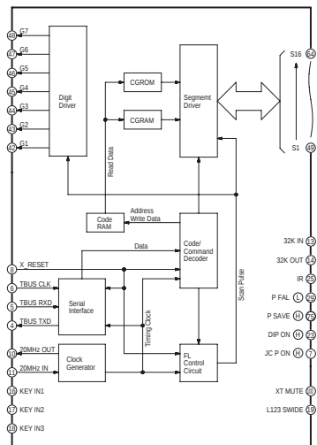
IC7501 TIMER IC-DETAIL BLOCK DIAGRAM
