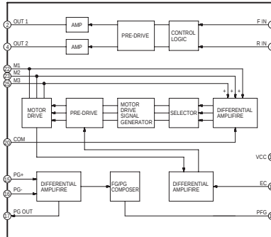
IC2501 LOADING/CYLINDER MOTOR DRIVE IC-DETAIL BLOCK DIAGRAM
