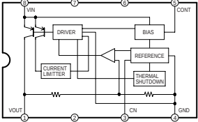
IC56104 +3.3V SWITCHING REG. IC-DETAIL BLOCK DIAGRAM
