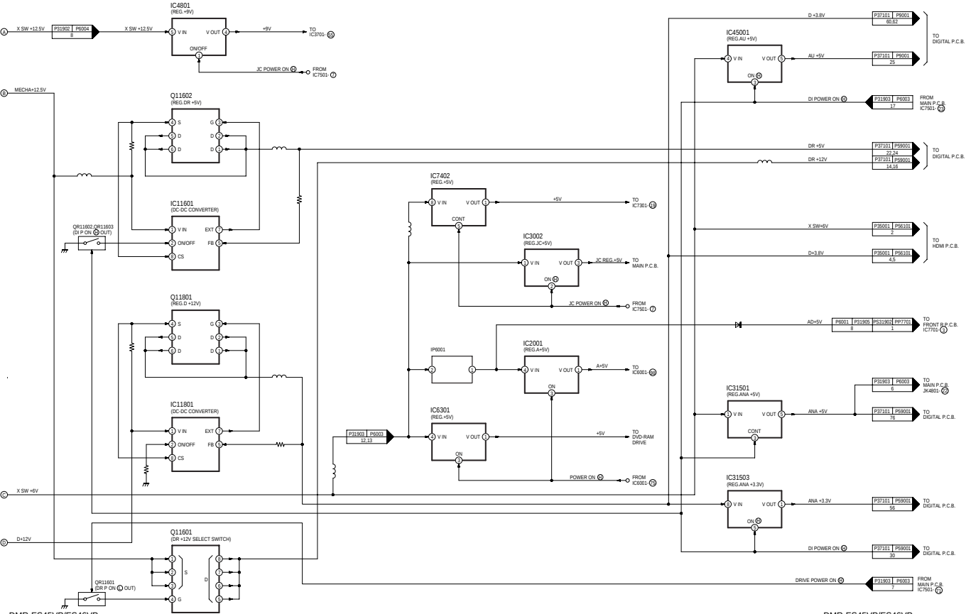
DMR-ES45VP/ES46VP Power Supply Block Diagram
