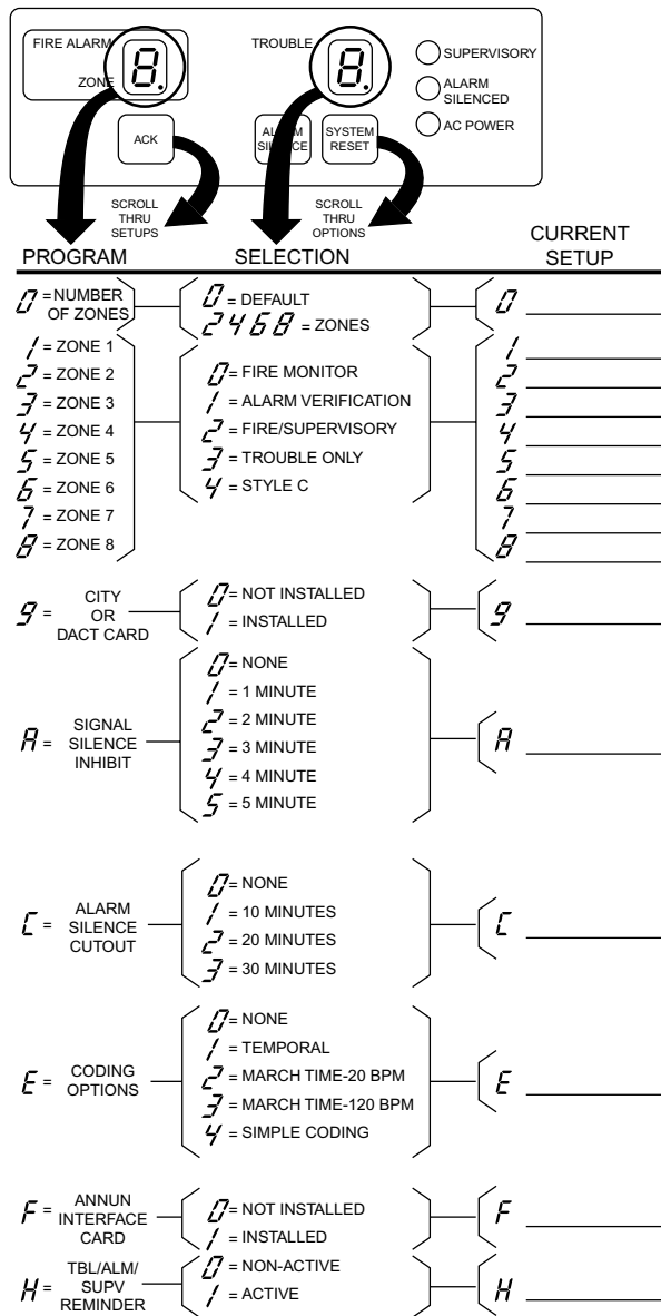
Figure 4. 4004 Programming Selections
