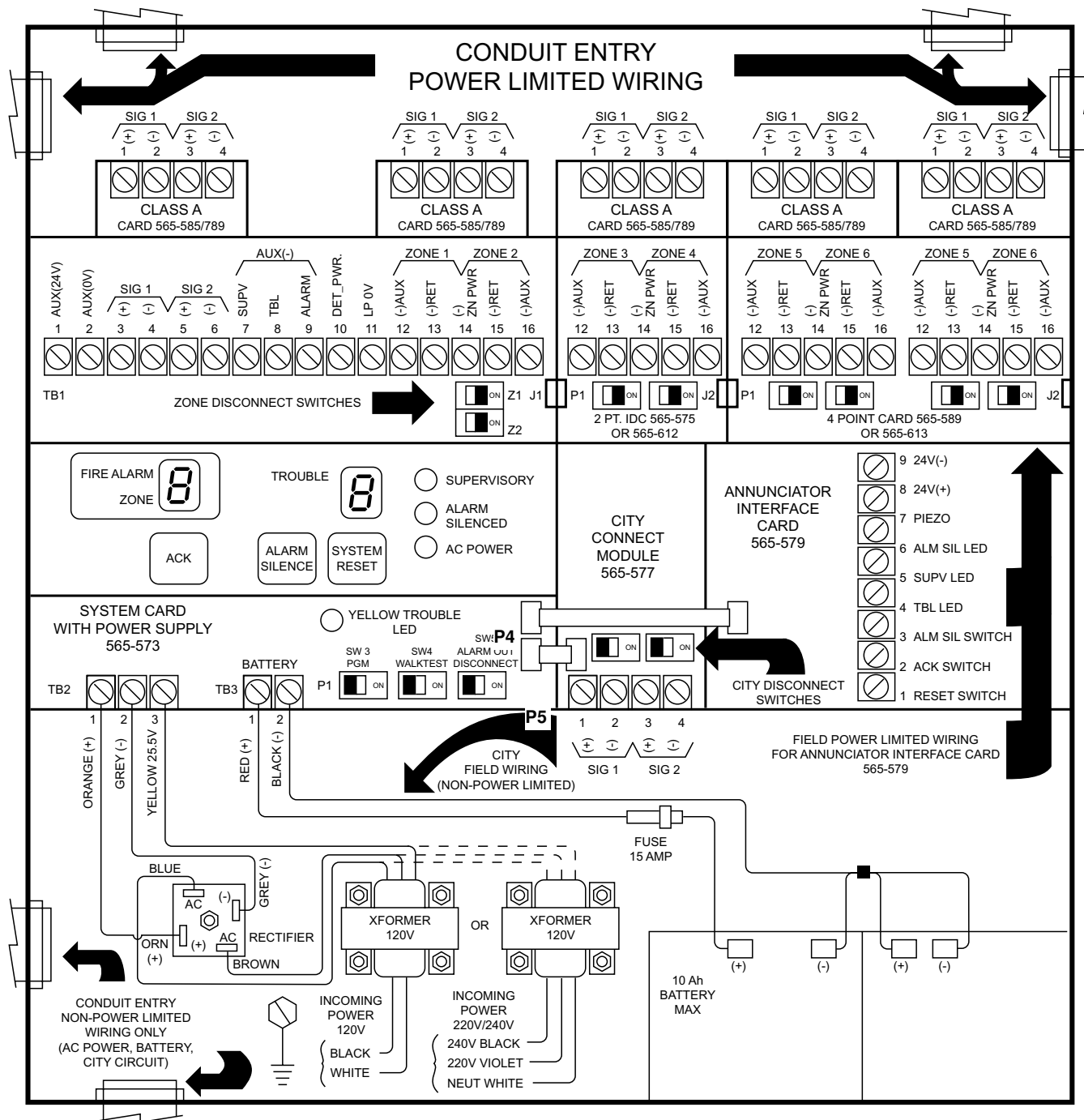
Figure 1. 4004 System Diagram
