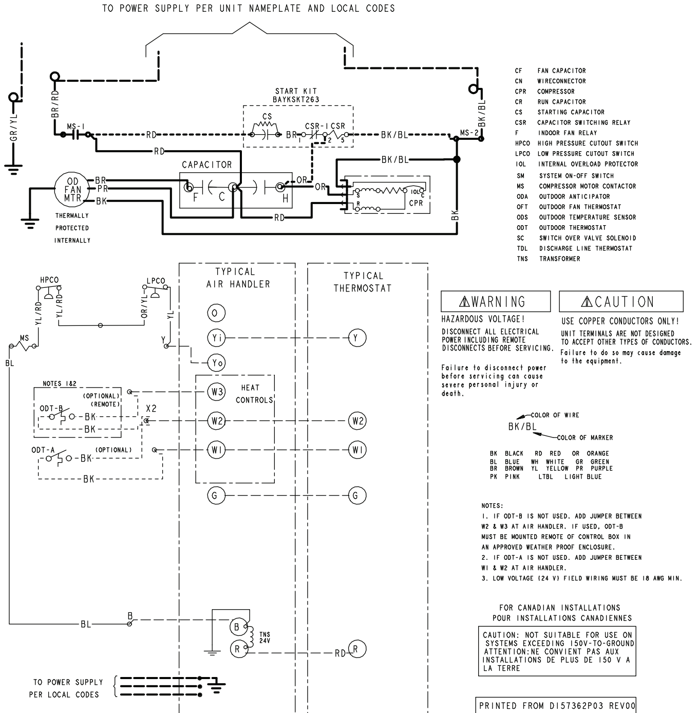
Figure 1. 1.5–4.0 Ton Models
