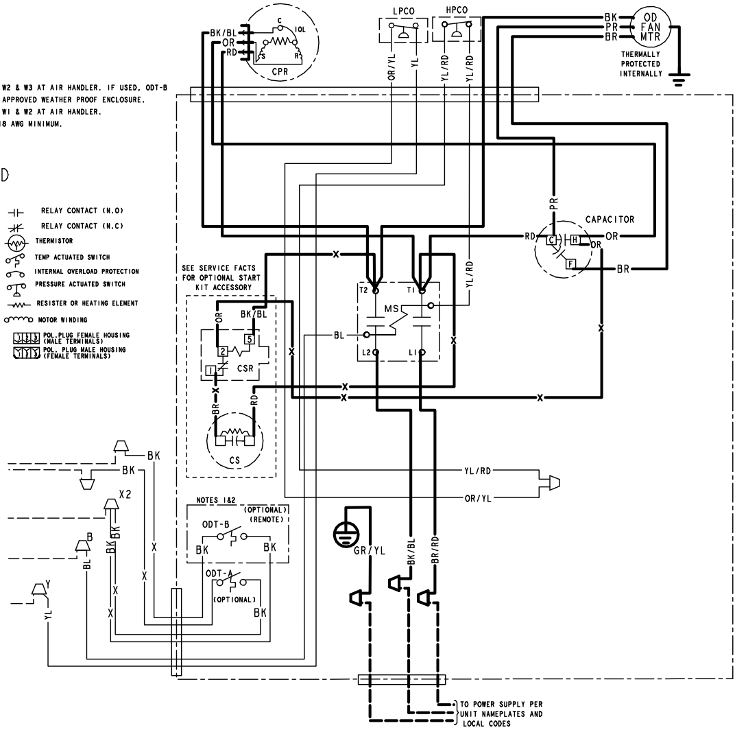
Figure 3. 5.0 Ton Models
