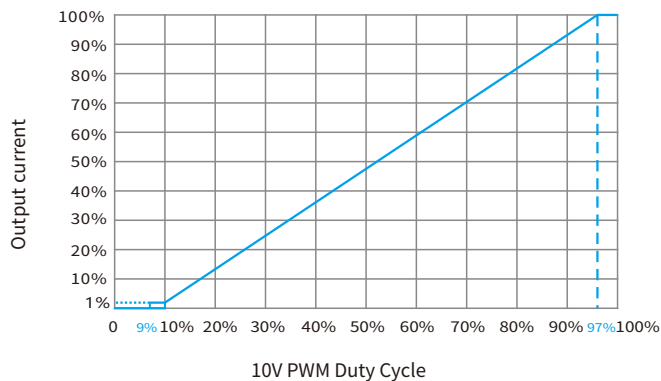
Output current 10V PWM Duty Cycle(Typical)
