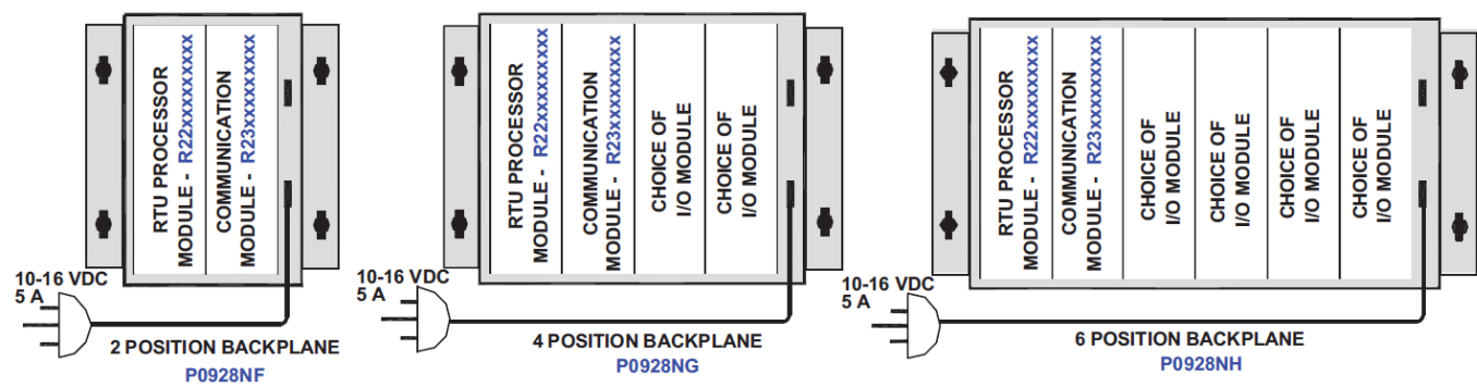
Figure 12 - Possible RTUs Using a BP-x Backplane
