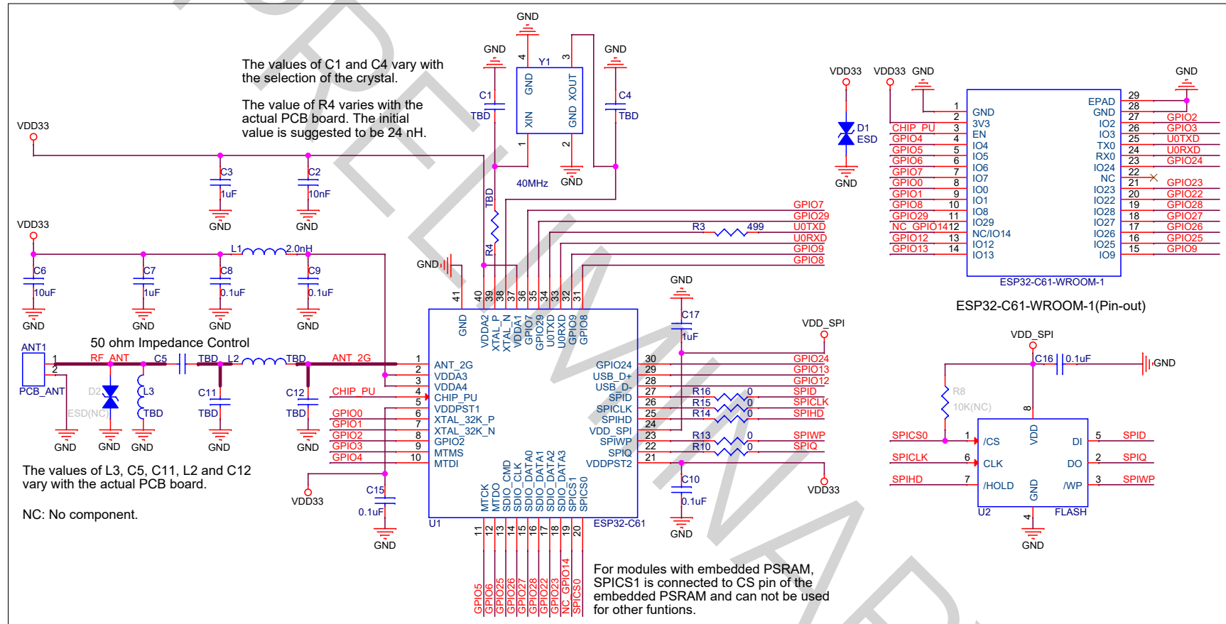
Figure 6: ESP32-C61-WROOM-1 Schematics
