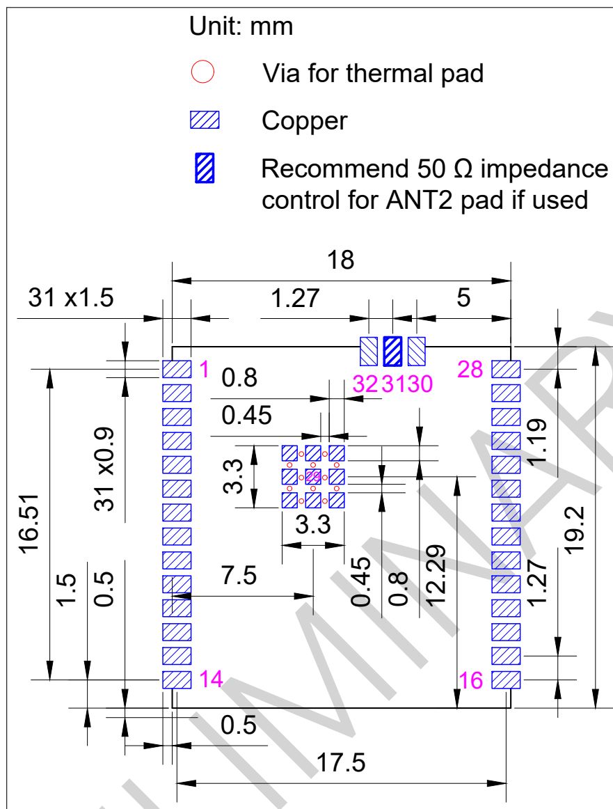
Figure 14: ESP32-C61-WROOM-1U Recommended PCB Land Pattern
