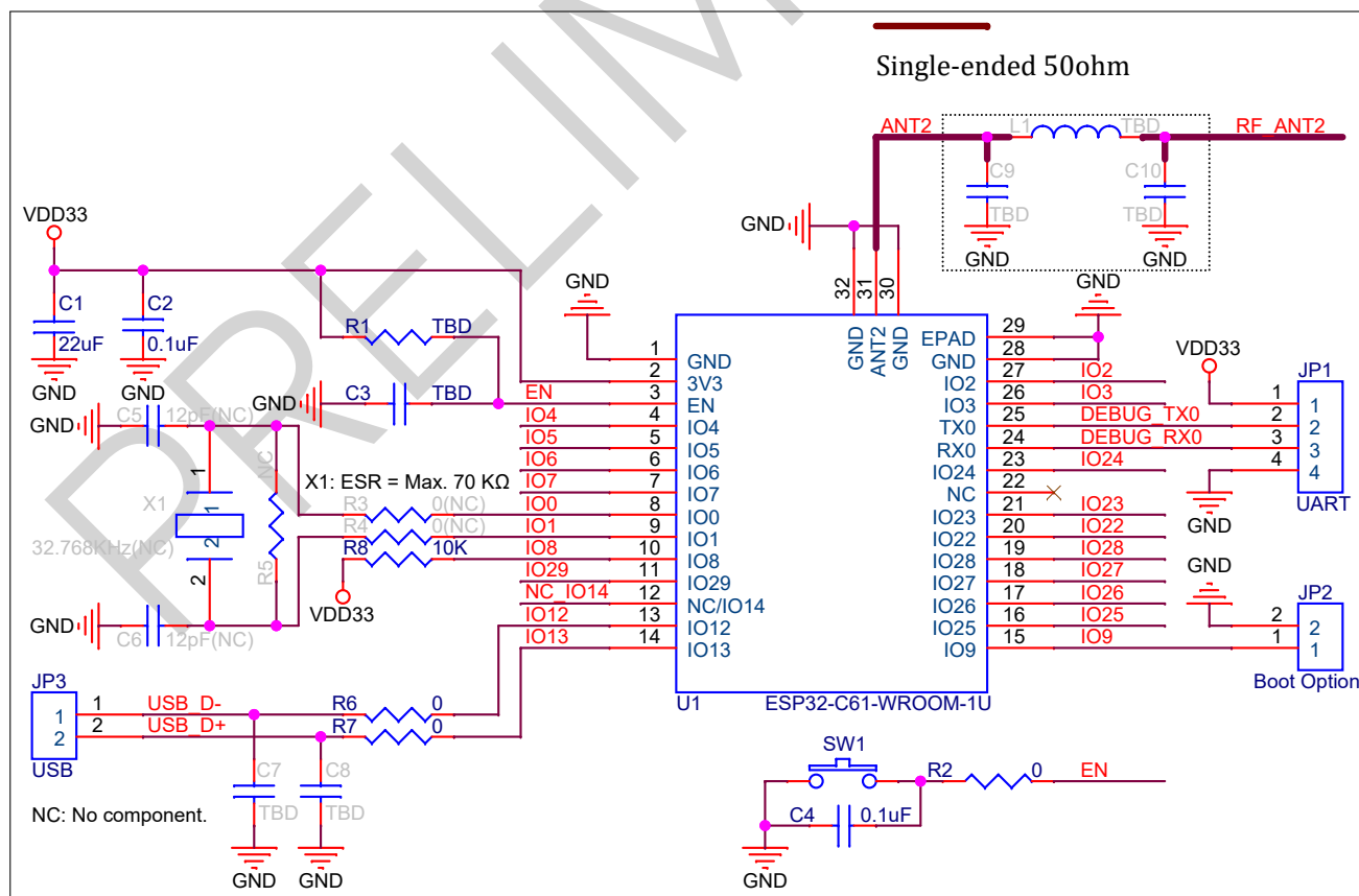
Figure 9: ESP32-C61-WROOM-1U Peripheral Schematics
