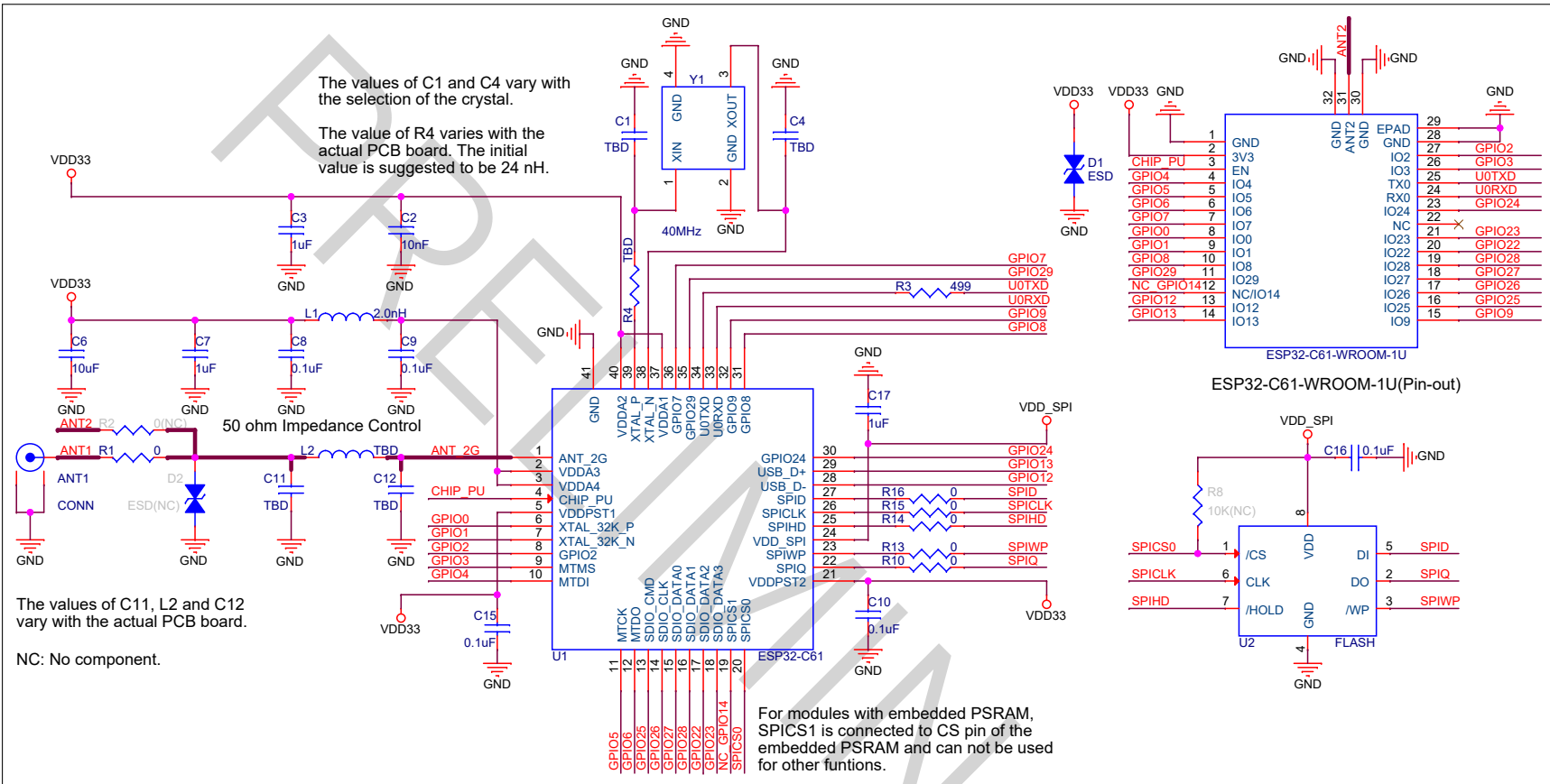
Figure 7: ESP32-C61-WROOM-1U Schematics
