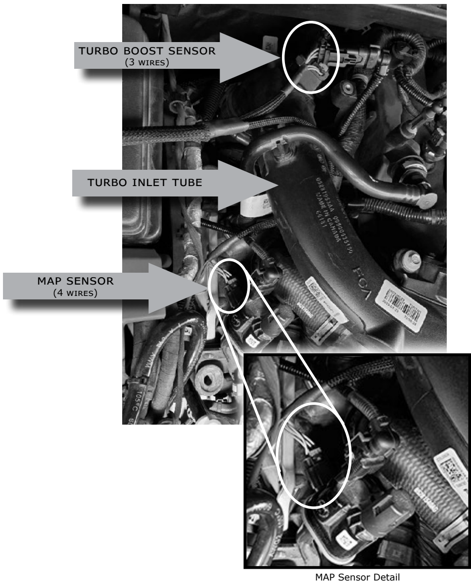
MAP Sensor Detail
