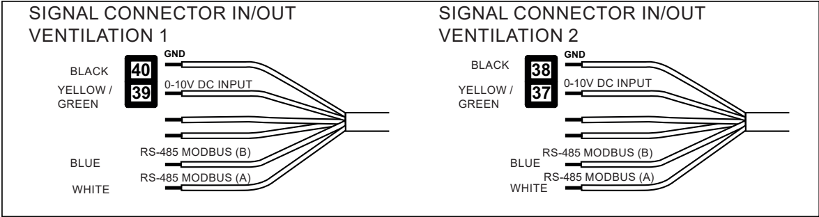
CONNECTION DIAGRAM WITH “VORT T PLUS” CONTROL UNIT (CODE 20.152)
