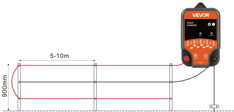
Three wire wiring diagram
