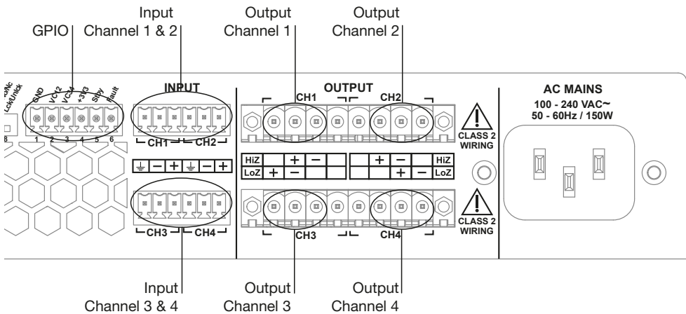
Diagram 6b PowerZone 1004 & PowerZone 504 connection sockets.
