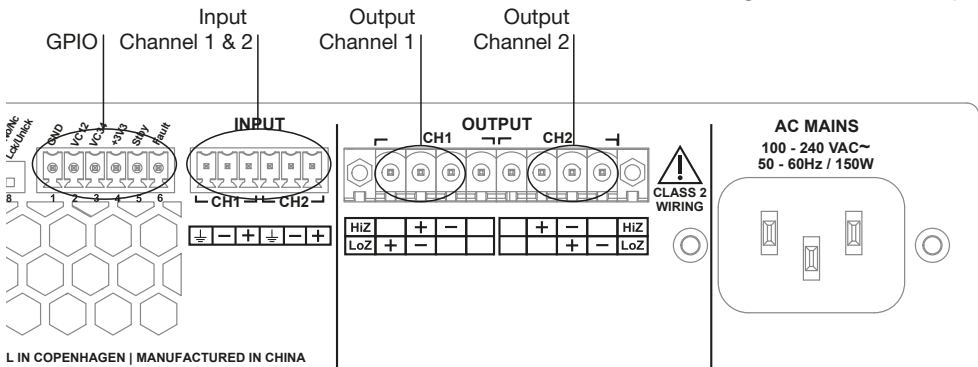
Diagram 6a PowerZone 252 connection sockets.
