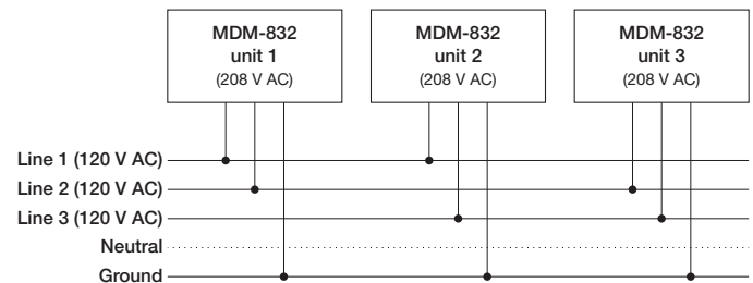
Figure 1: 120 V AC, 3-Phase Wye System (Two Lines to Each MDM-832)
