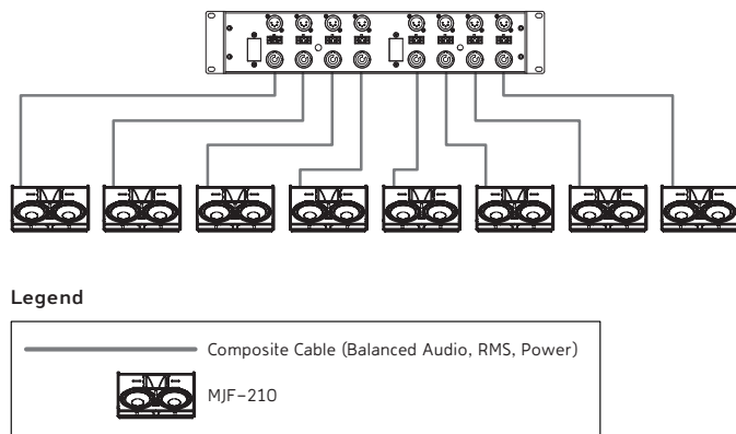
MDM-832 Connected to Loudspeakers with Composite Cables
