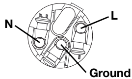
powerCON 20 Terminals
