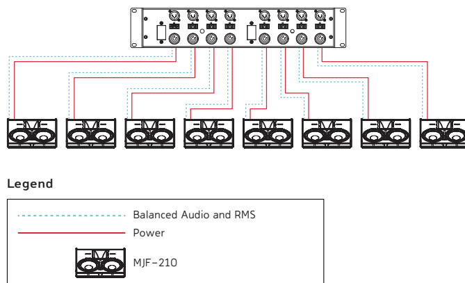
MDM-832 Connected to MJF-210 Loudspeakers with Separate Cables
