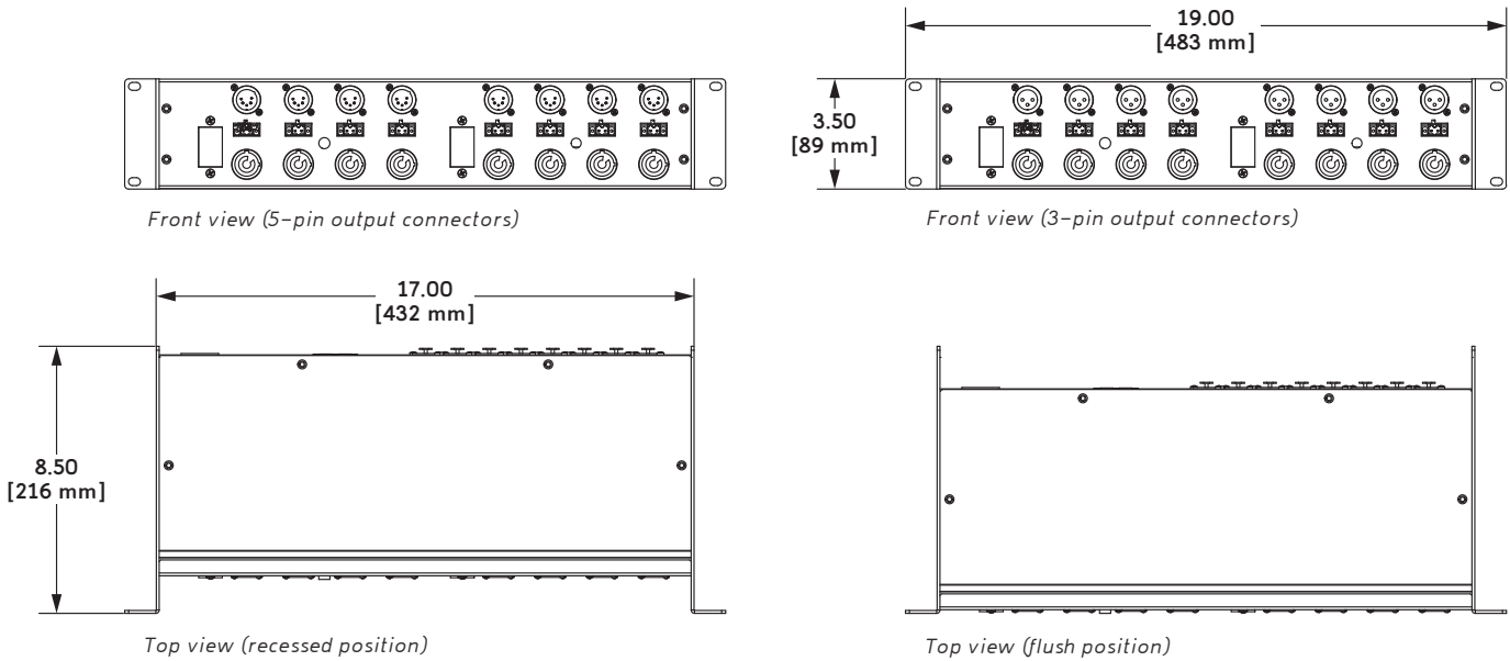
MDM-832 Dimensions
