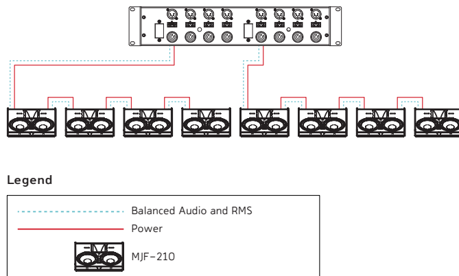
MDM-832 Connected to MJF-210 Loudspeakers with Separate Cables and Loop Outputs
