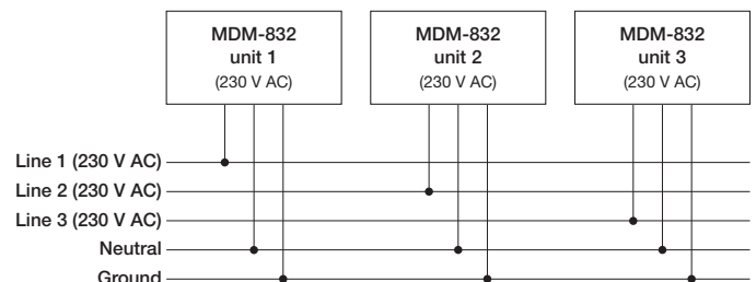
Figure 2: 230 V AC, 3-Phase Wye System (One Line to Each MDM-832)
