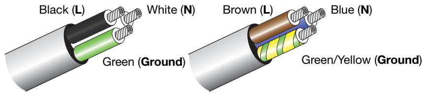
Power Cable Colors
