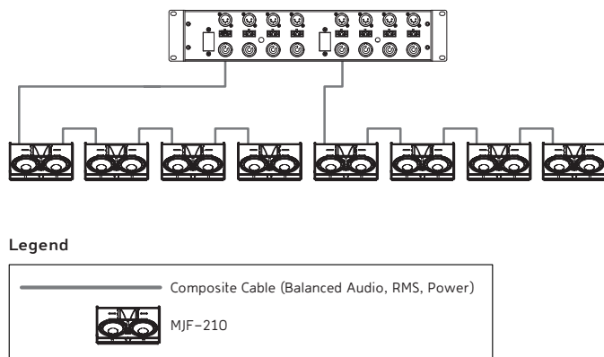
MDM-832 Connected to Loudspeakers with Composite Cables and Loop Outputs
