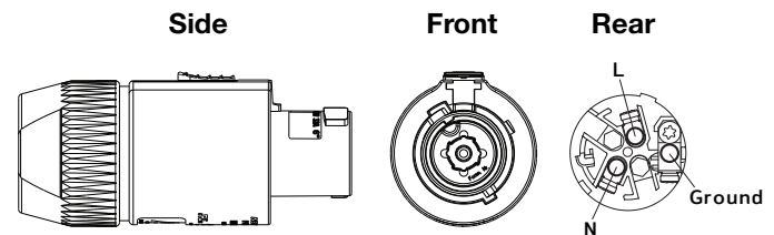
powerCON 32 AC Input Connector
