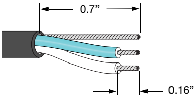
Signal Pair Exposed Lengths
