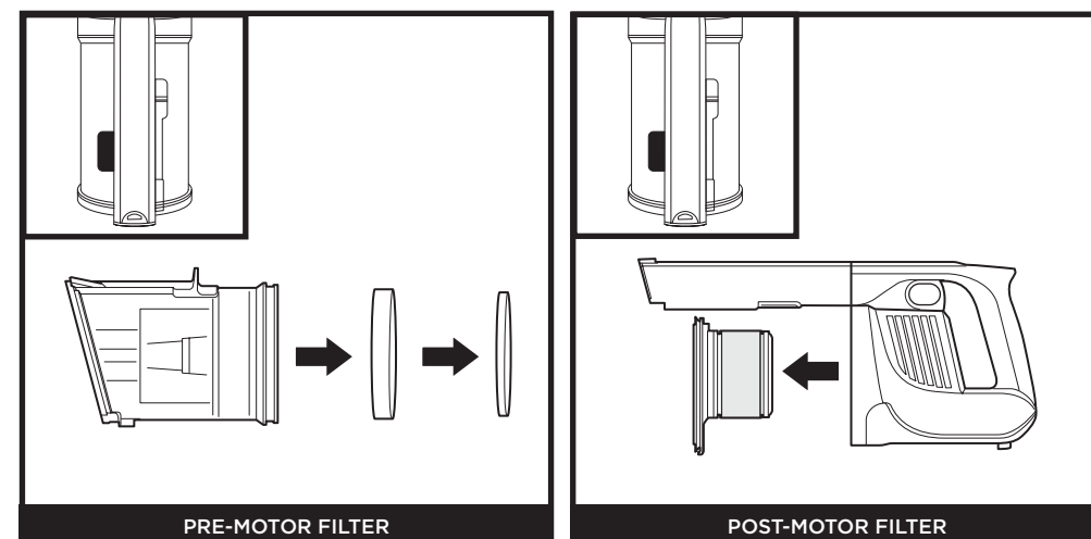
PRE-MOTOR FILTER
