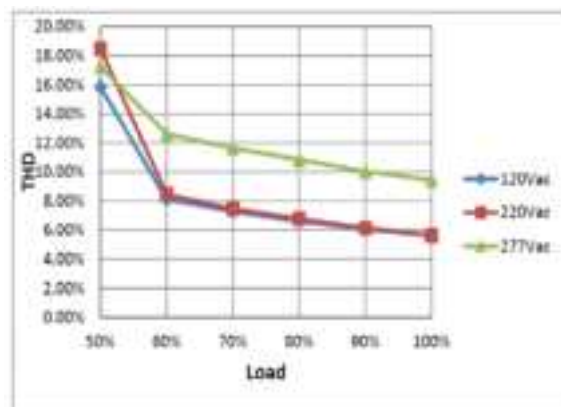
THD Curve
