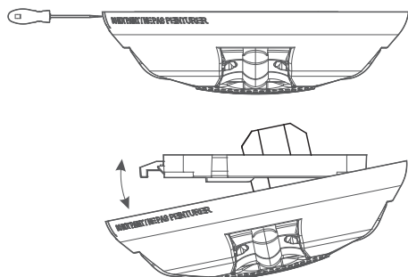
Removing Device
