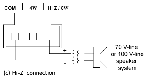
(c) Hi-Z connection
