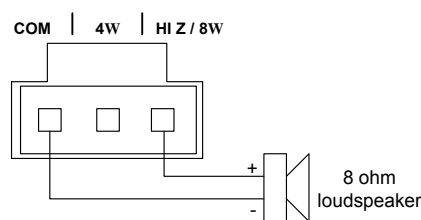
(b) Lo-Z (8 ohm) connection
