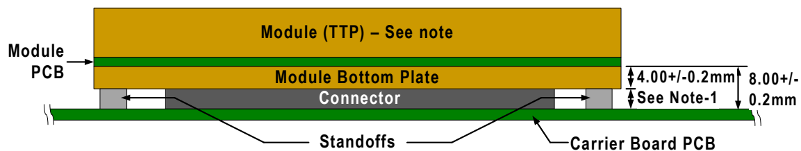
Figure 3-3. 5.5 mm Height on Carrier Board
