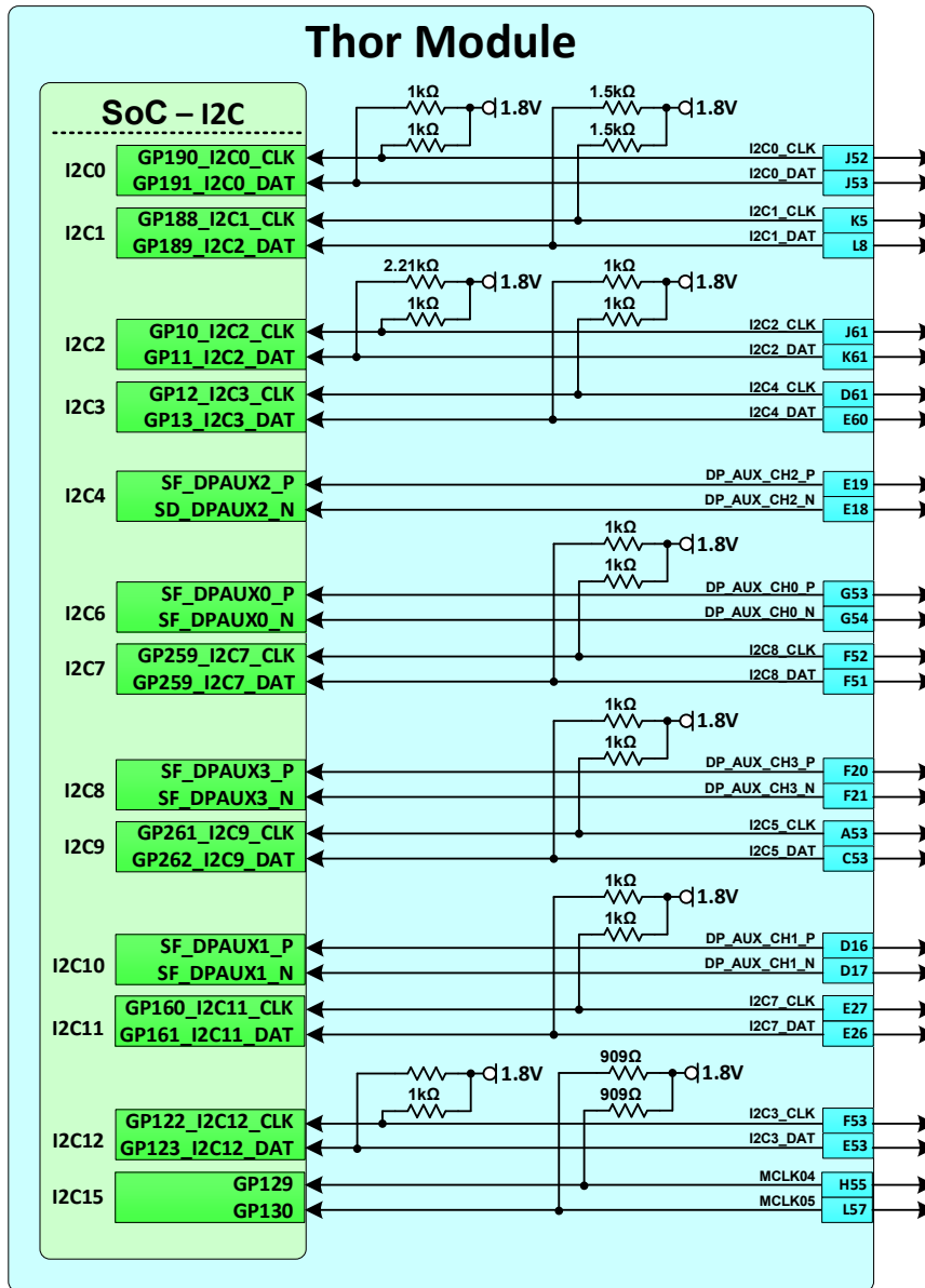
Figure 12-1. I2C Connections
