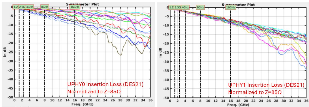
Figure 7-9. Insertion Loss S-Parameter Plot (DES21)
