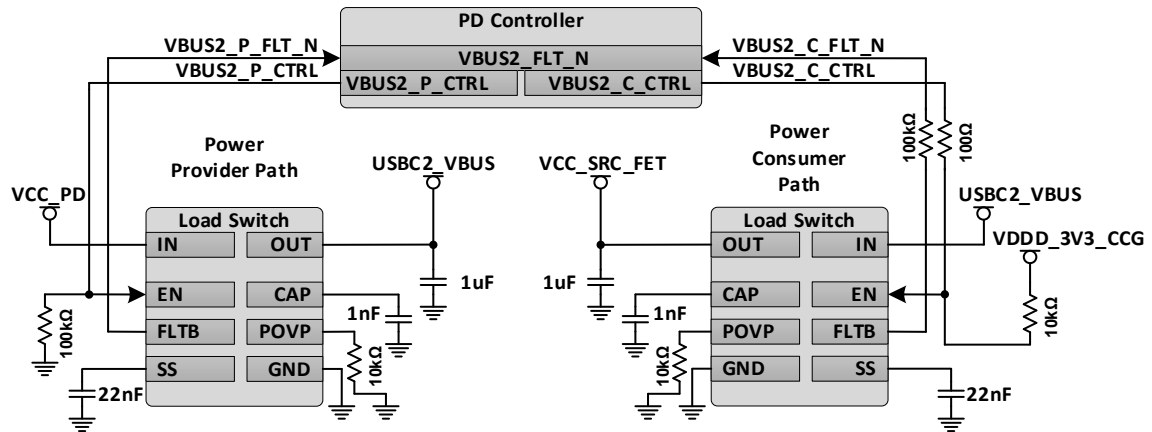
Figure 7-4. USB Type-C Dual Mode Circuitry Sample Connections
