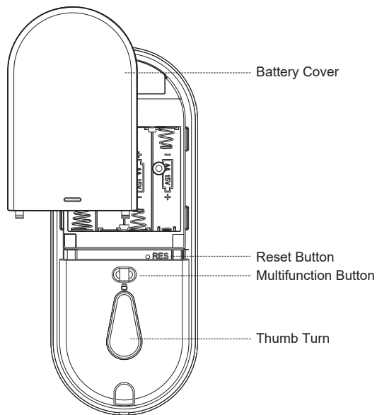
Interior Assembly
