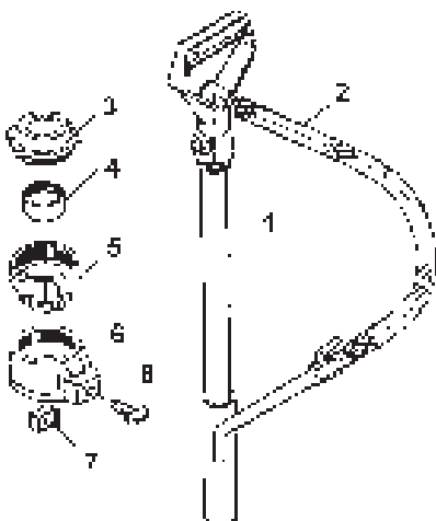
fig.1 TP67 Gear Oil Pump
