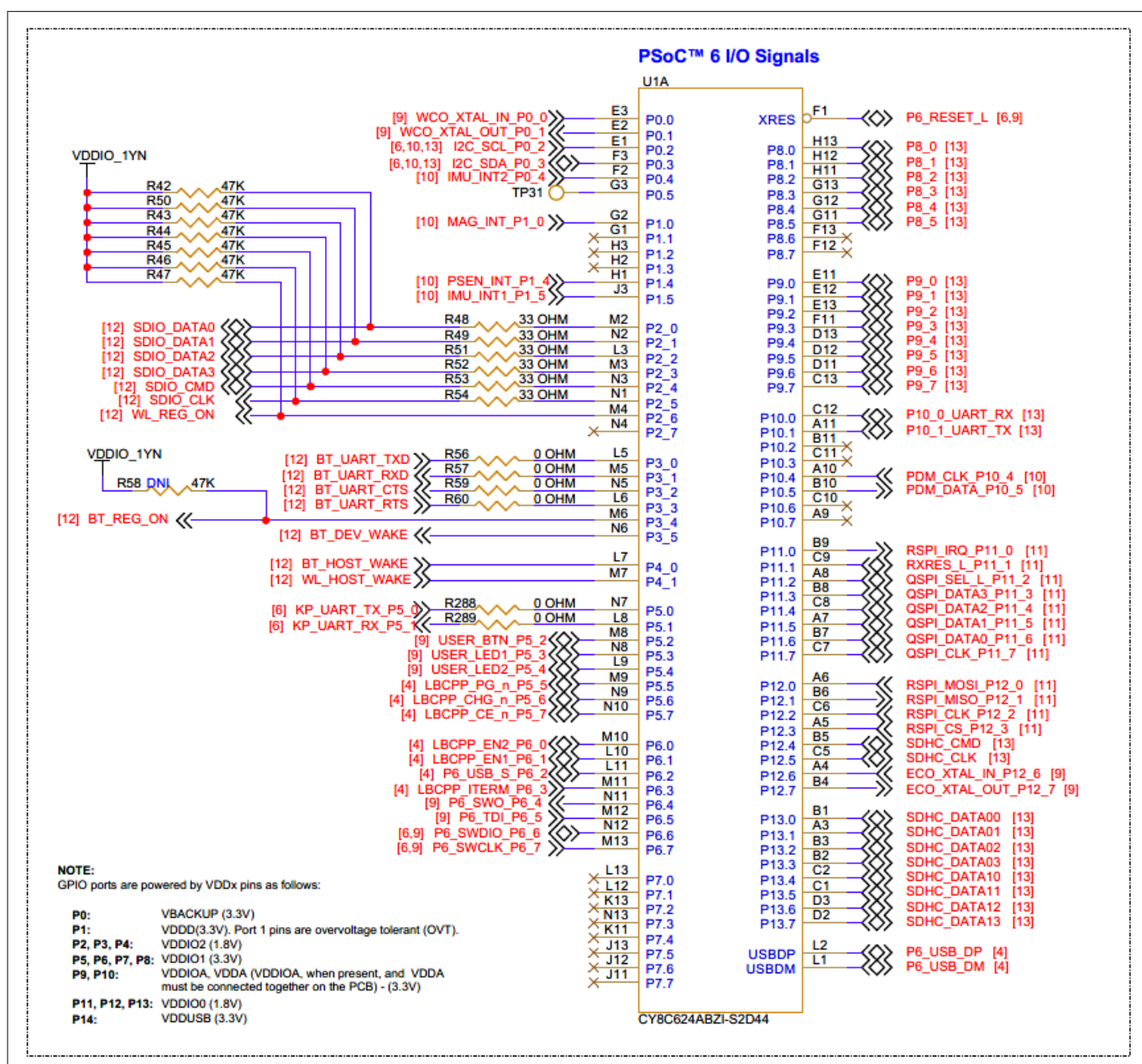
Figure 23 Schematic of PSoC™ 6 MCU IO signals
