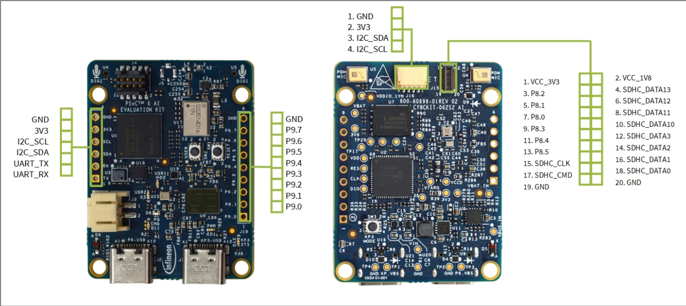
Figure 2 Board pinout
