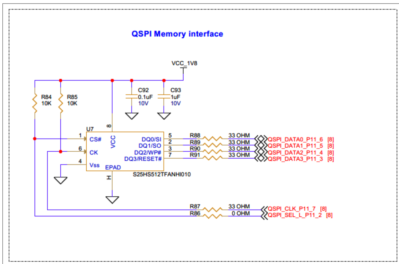
Figure 38 Schematic of QSPI flash memory interface
