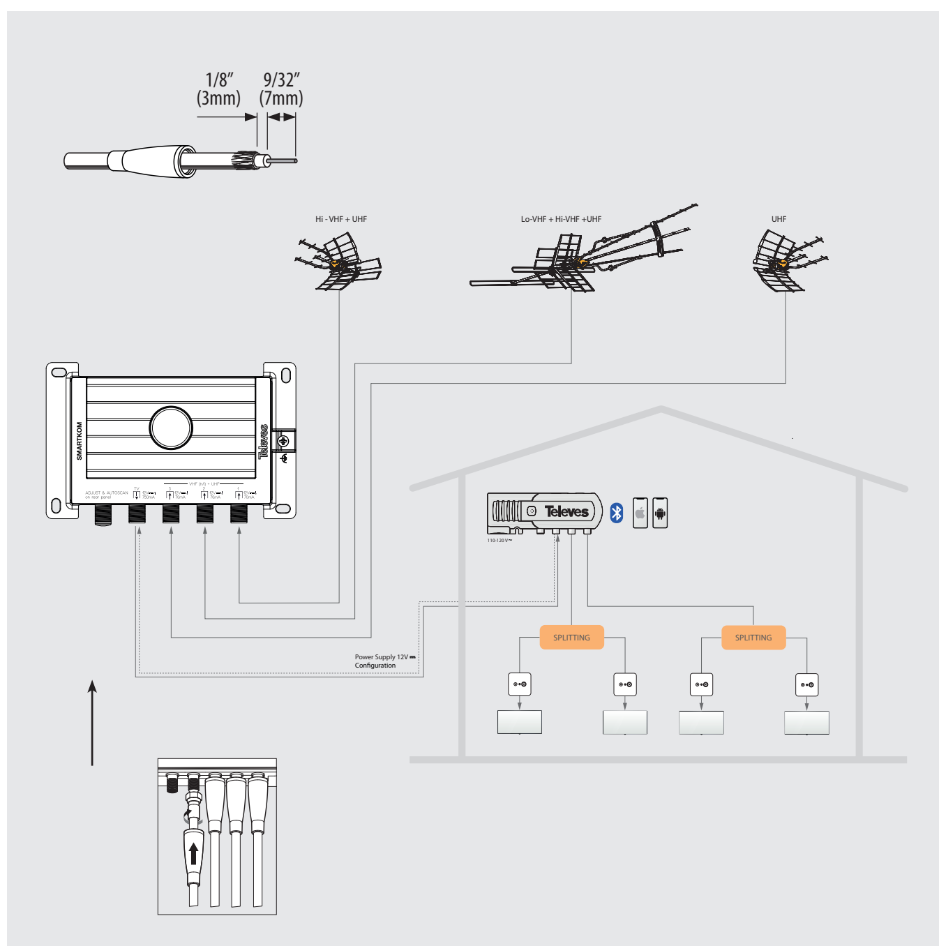
Figure 3: Application example
