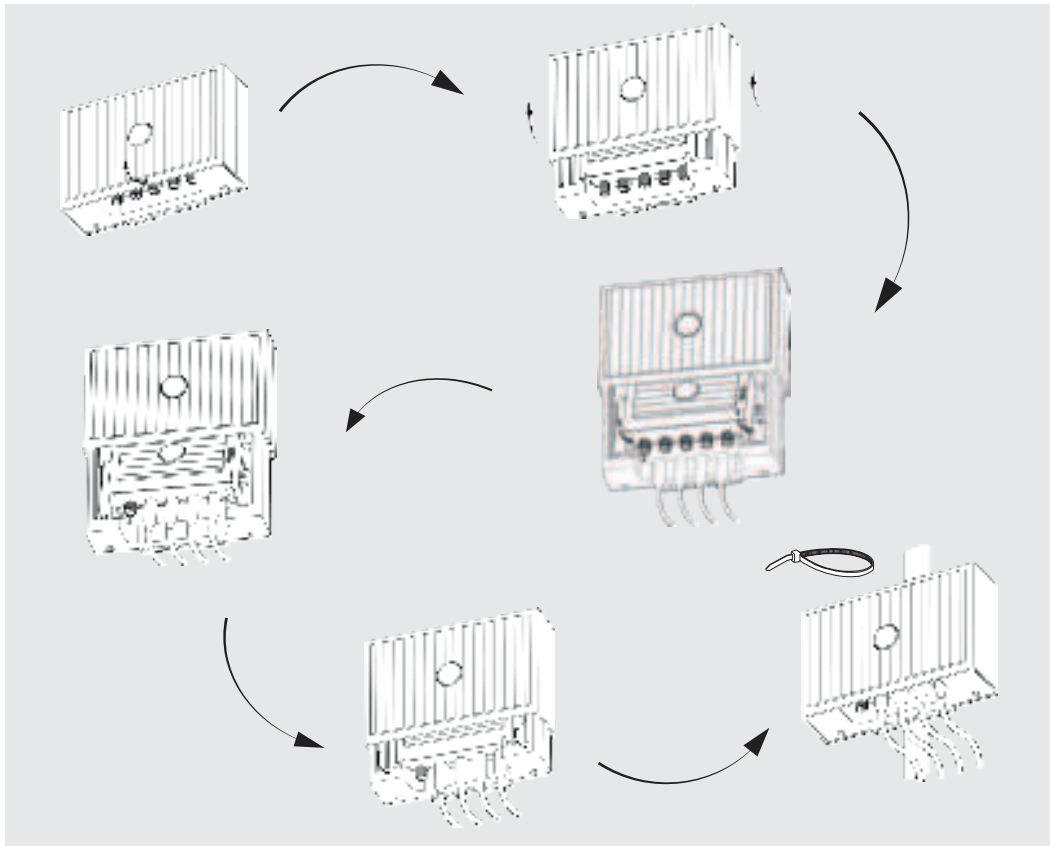
Figure 4: Installation example
