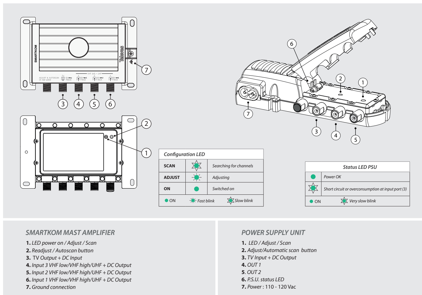
Figure 1: Connections and controls
