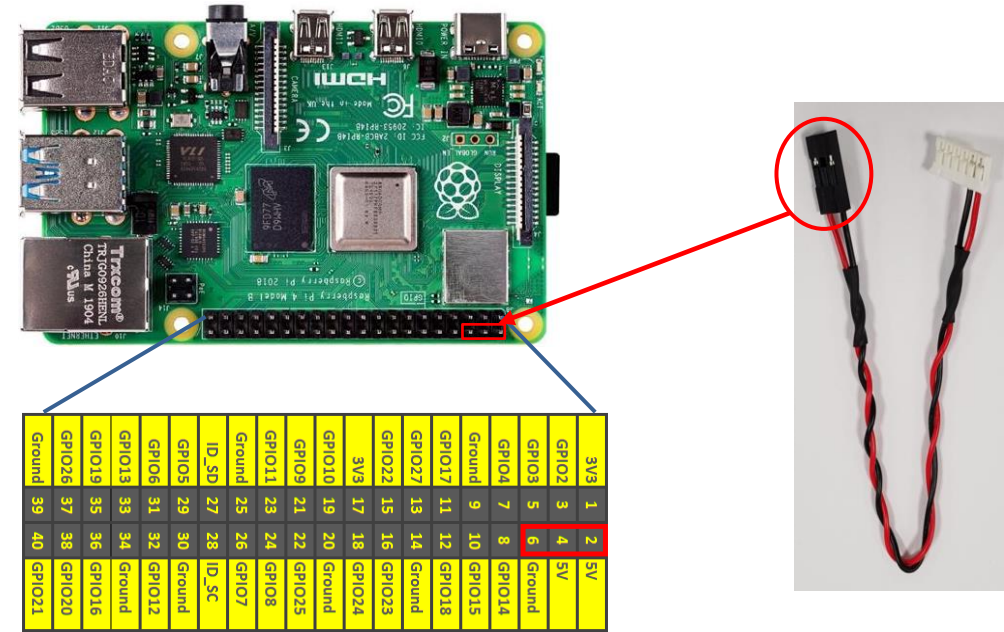
Item#5 – Internal Power Connector
