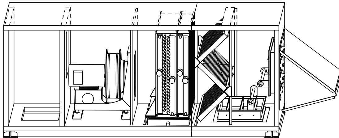
Figure 11. Outdoor unit with DDP fan configuration
