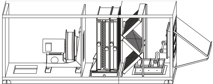
Figure 2. Direct-drive fan/mixing box with bottom discharge — horz draw-thru
