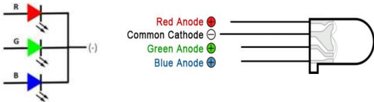
Common Cathode (-)
