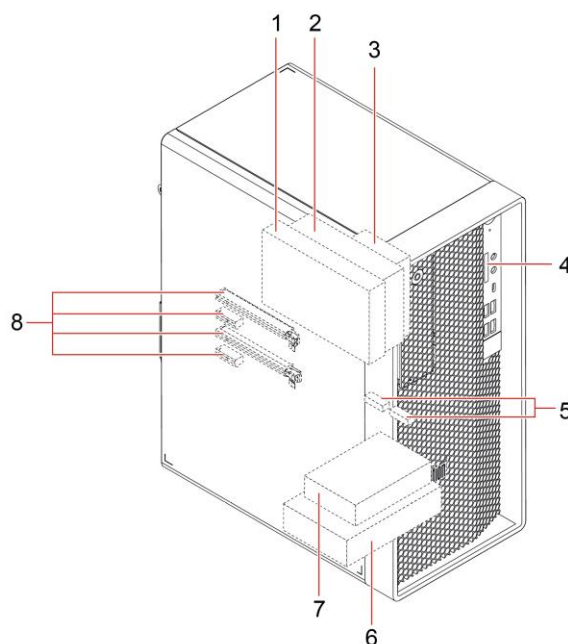
Figure 4– P2 Tower Gen 2 Storage location layout
