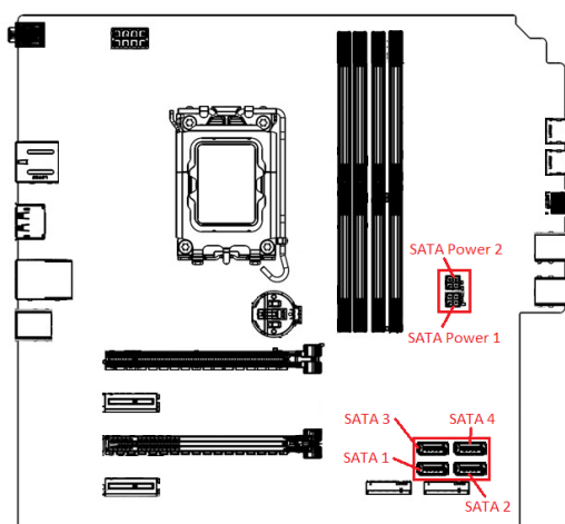
Figure 3 – P2 Tower Gen 2 Motherboard with SATA ports Locations-Callouts
