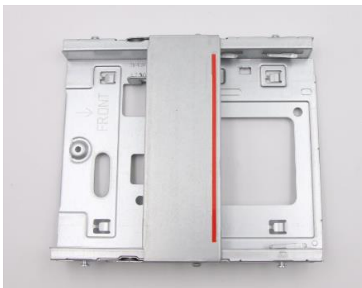
Slim ODD Bracket Assembly (Tower only)
