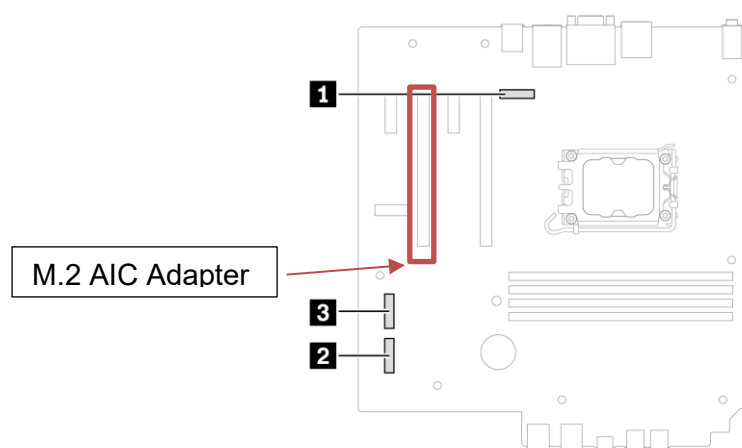
Figure 1 – P2 Tower Gen 2 Motherboard Diagram with NVMe Locations
