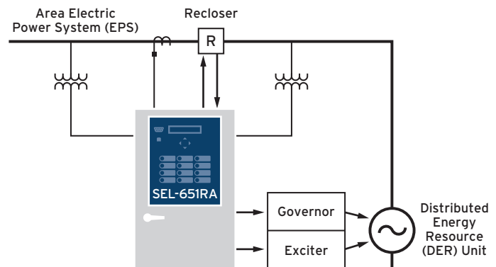
Typical utility and DER interconnection.
