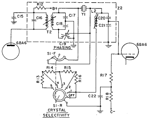
Fig. 3—Crystal Filter Circuit.
