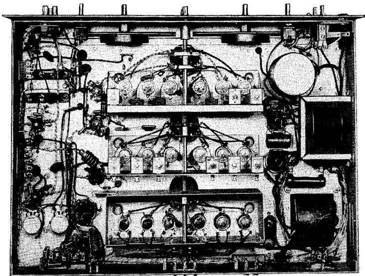
Fig. 6--Bottom view showing placement of parts.
