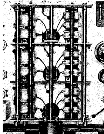
Fig. 4—H. F. Tuning Assembly.
