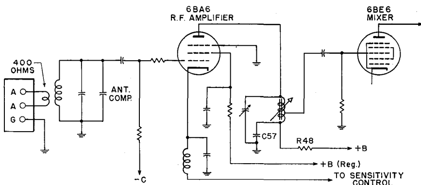
Fig. 2—Tuned RF Amplifier and Mixer.
