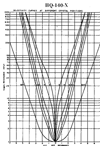
Fig. 10—Selectivity Curves.
