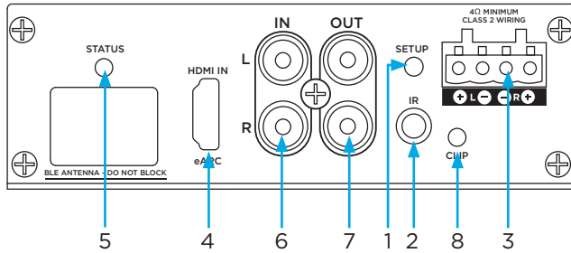
UA 2-125 ARC Amplifier Audio Connector Panel
