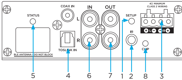
UA 2-125 Amplifier Audio Connector Panel
