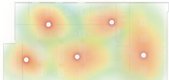
Reasonable AP Deployment with Wi-Fi Heatmap Simulator
