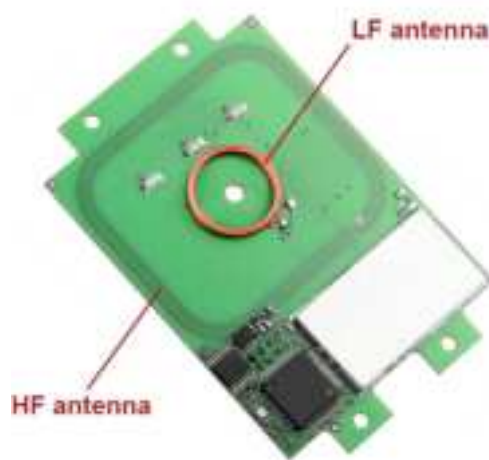
TWN4 MultiTech 2 LEGIC M LF HF (exemplary picture)
