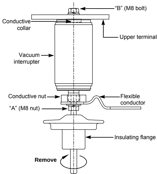
Figure 12: Removing the Vacuum Interrupter
