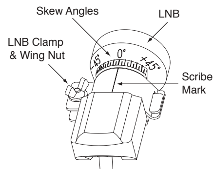
Figure 5-7 LNB Skew Angle Setting (European Systems Only)
