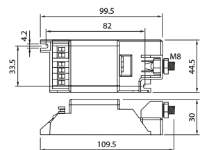
Afmetingen DD-SELV in mm.
