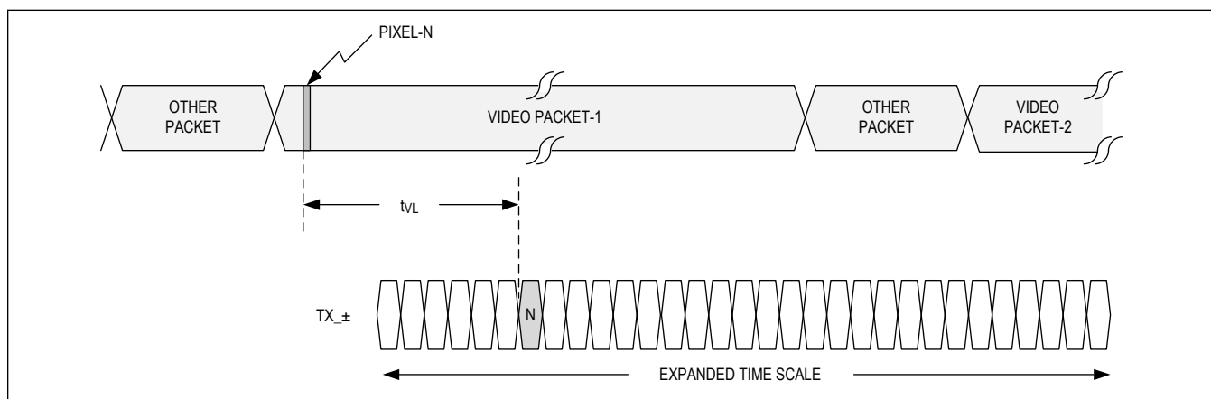
Figure 3. Video Latency
