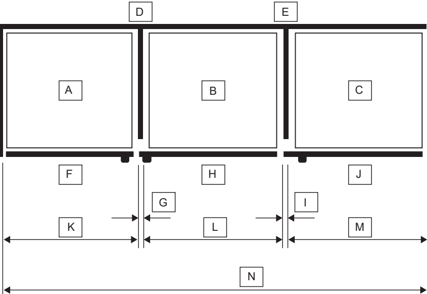
Diagram B – Smallest Cutout (Door Opening is Restricted) Applies to Custom Panels Only.
