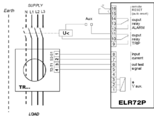
ELR72P - undervoltage release wiring
