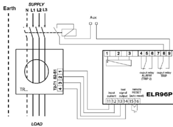
ELR96PF - shunt trip wiring
