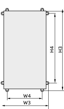
Front view Wall-mounting cabinet Wall fastening dimensions
