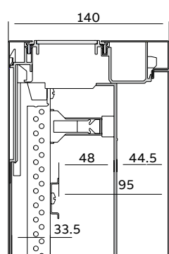
Compact distribution board panel
