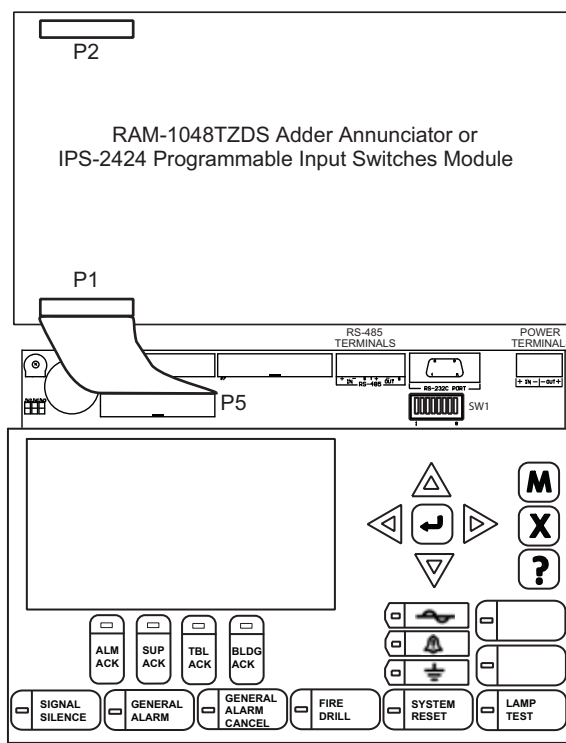
RAXN-LCDG GRAPHIC ANNUNCIATOR BOARD
