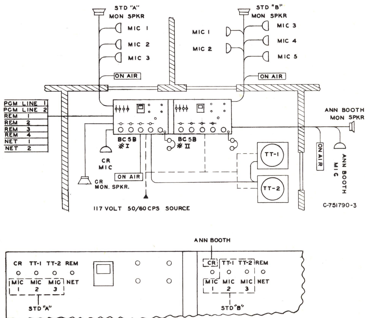
Figure 19—Typical Layout for Two-Studio Operation Control Room
