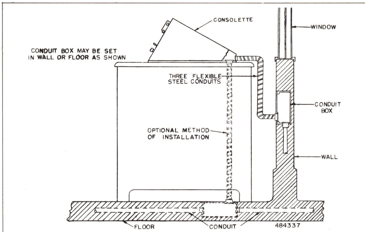
Figure 15—Typical Installation Showing Cable Installation for Consolette
