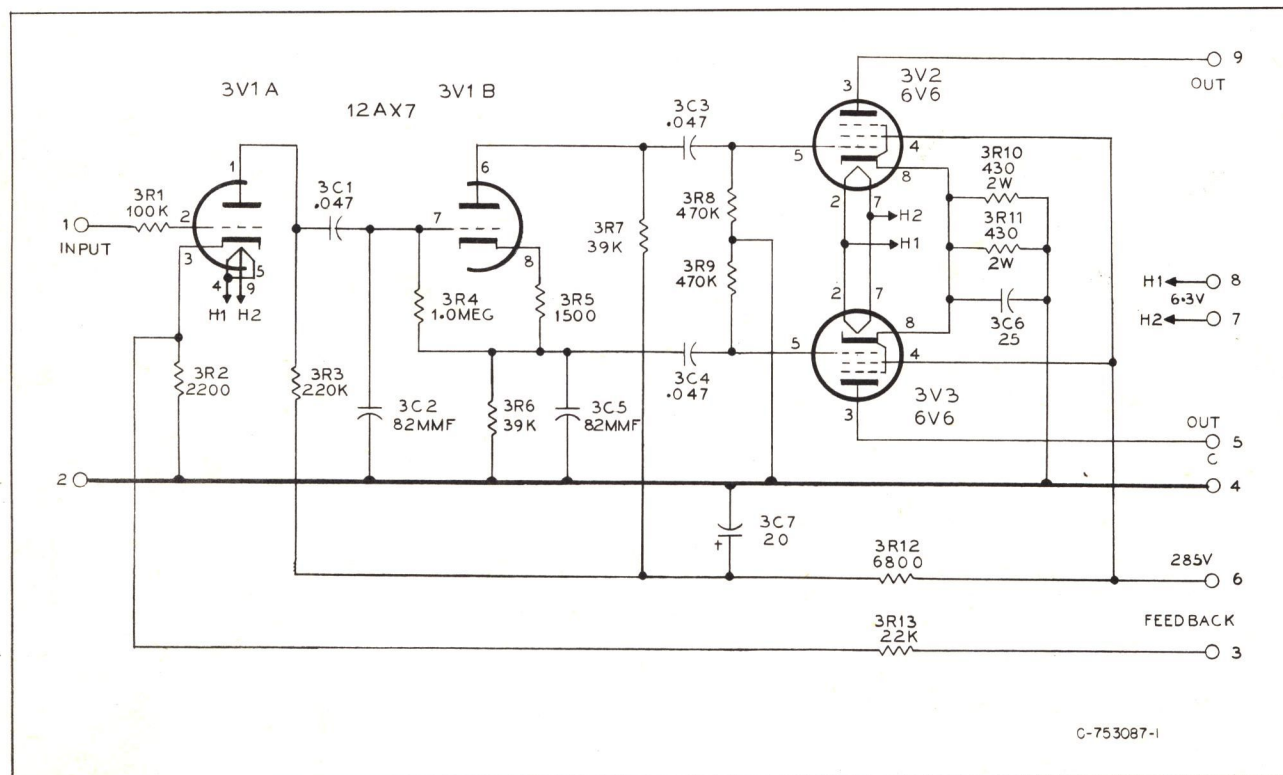
Figure 10—Schematic Diagram for Monitor Amplifier
