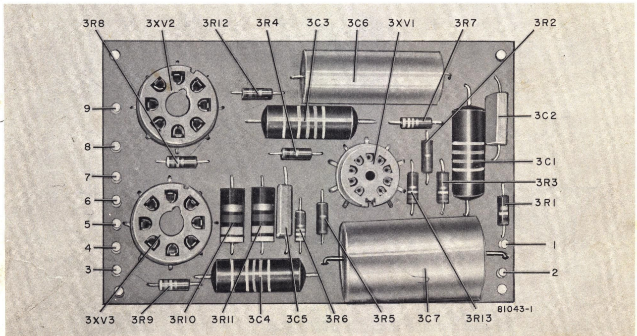
Figure 8—Monitor Amplifier 5AR8 Printed Circuit Board
