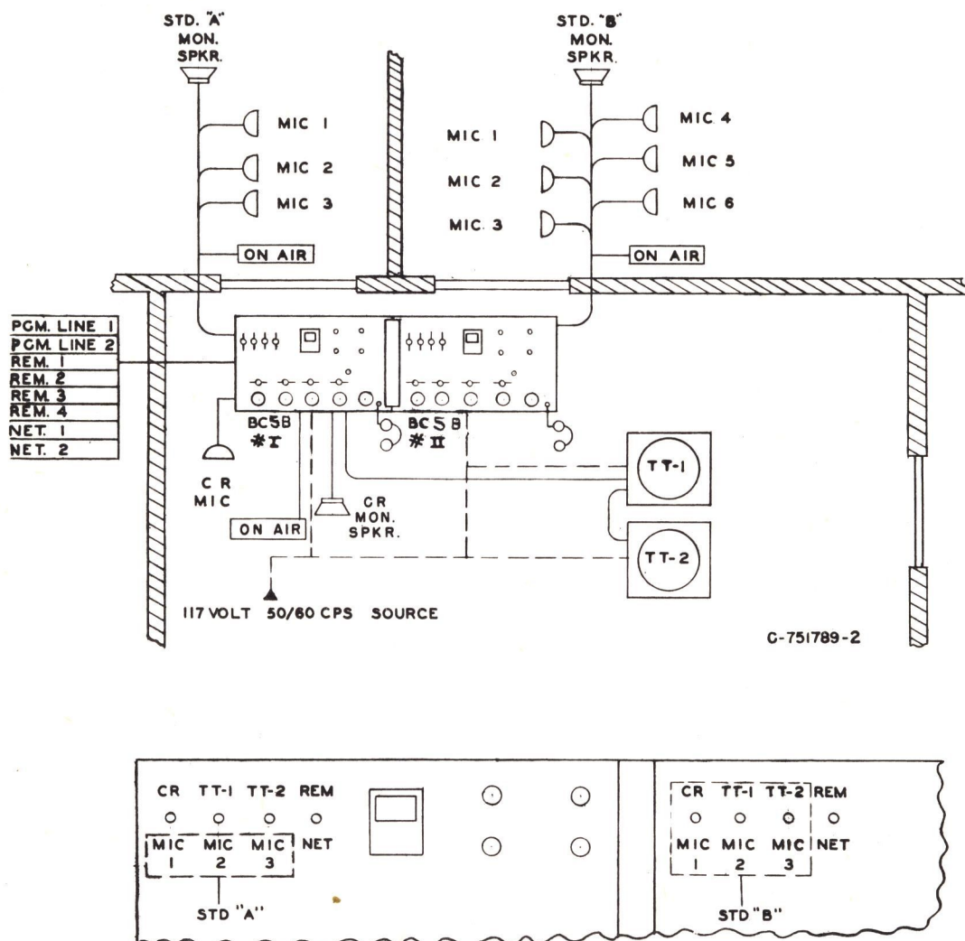
Figure 18—Typical Layout for Two-Studio Operation with Control Room and Announce Booth
