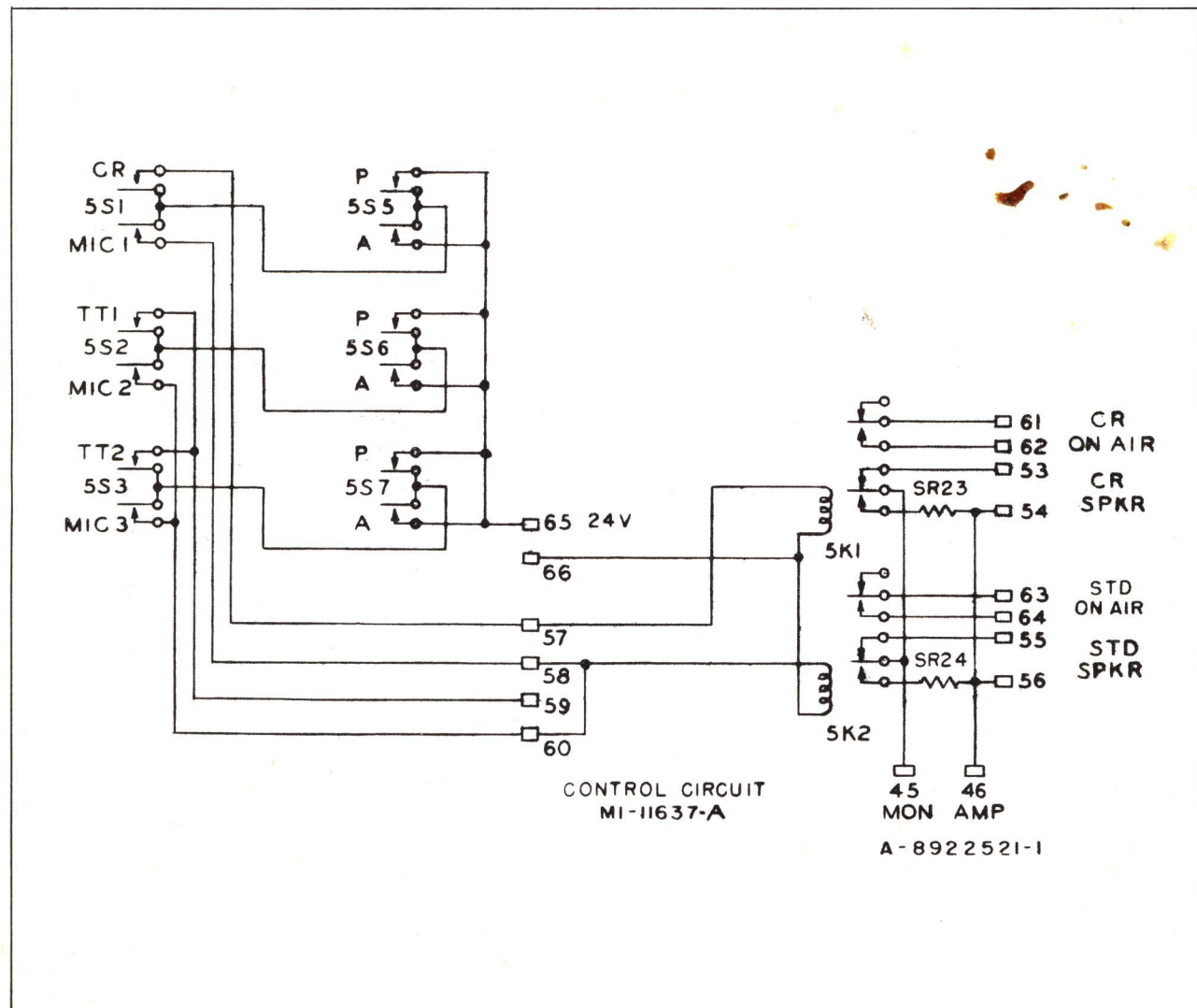
Figure 21—Control Circuit
