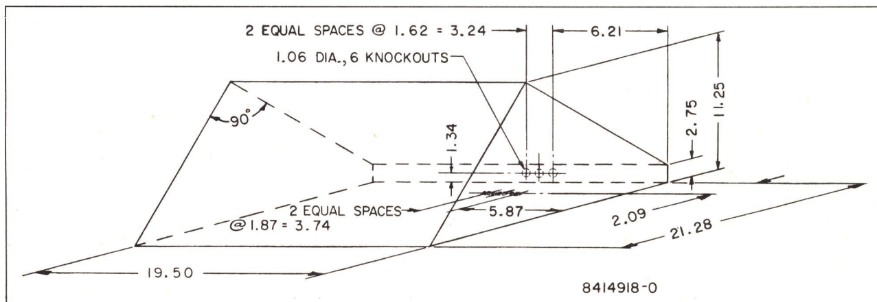
Figure 16—Installation Dimensions
