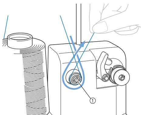
① Tension disc
