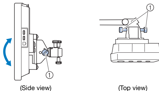
① Thumb screws
