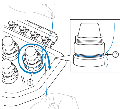
① Thread tension disc
