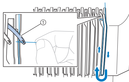
① Thread take-up lever
