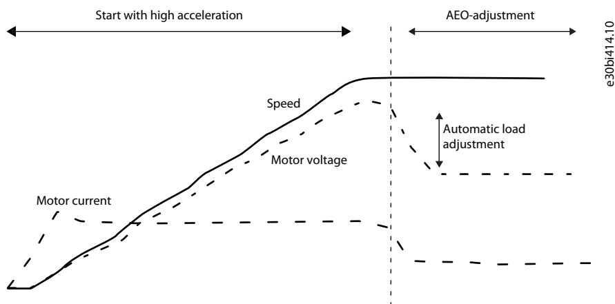
Illustration 10: Automatic Energy Optimization
