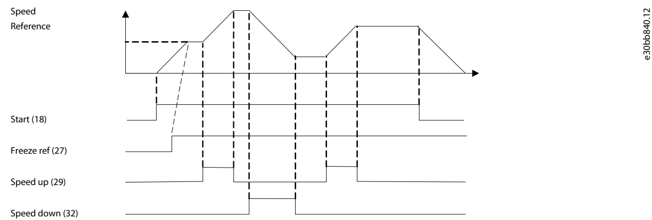
Illustration 97: Speed Up/Down
