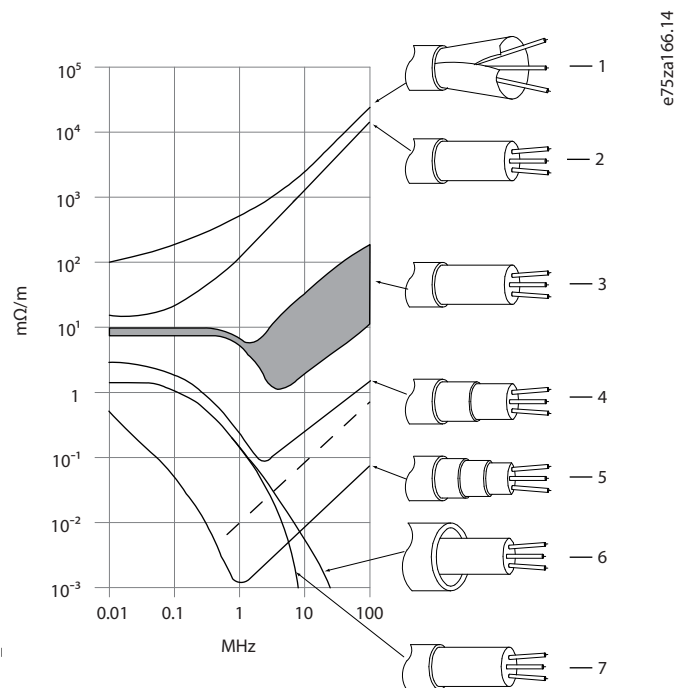
Illustration 62: Transfer Impedance ( Z_T )
