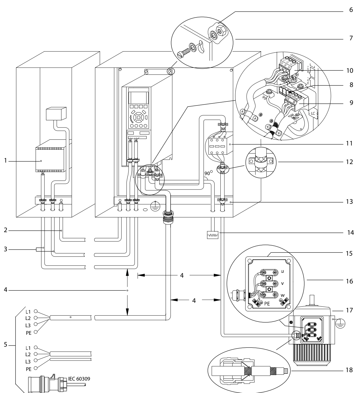
Illustration 82: Example of Proper EMC Installation
