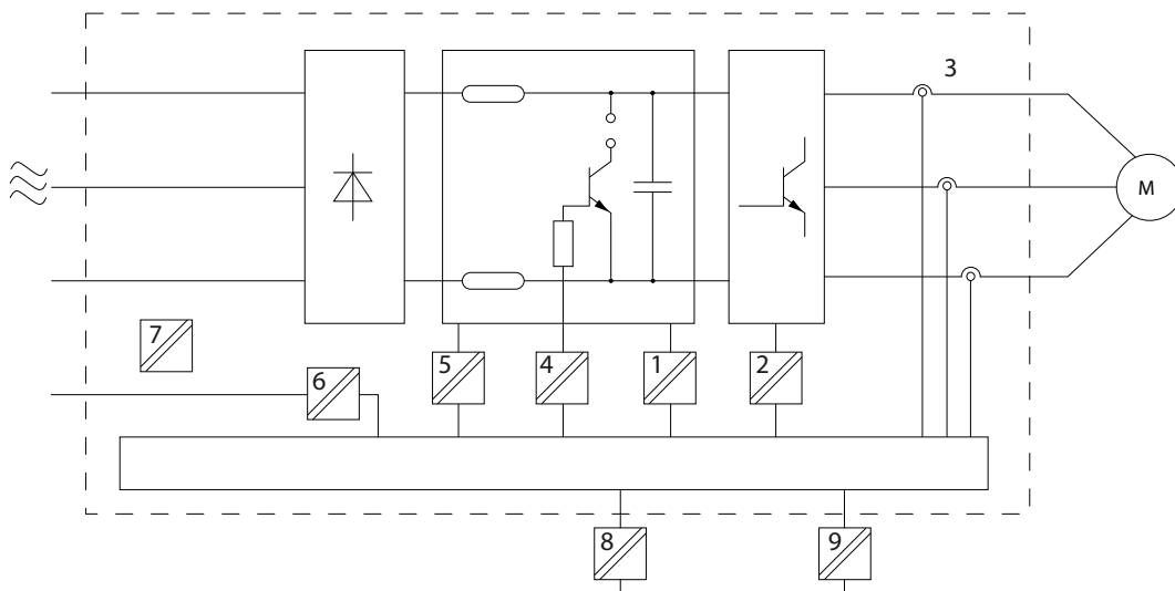
Illustration 81: Galvanic Isolation
