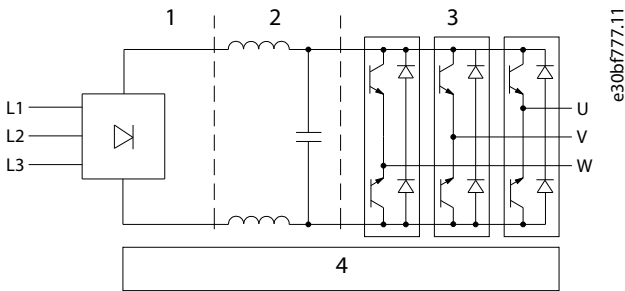
Illustration 87: Internal Processing
