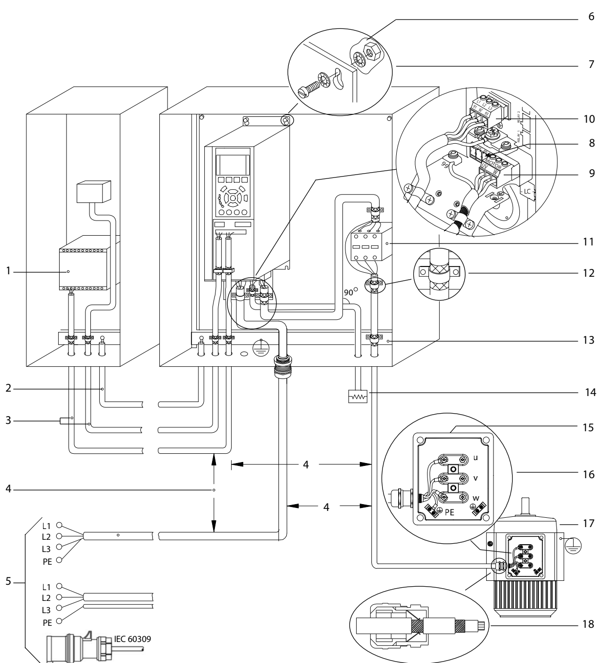
Illustration 61: EMC-compliant Electrical Connection
