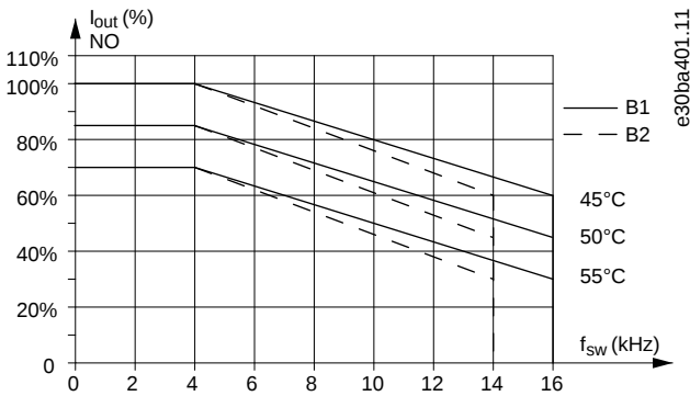
Illustration 44: Derating of I_{out} for Different T_{AMB,MAX} for Enclosure Sizes B1 and B2, using 60° AVM
