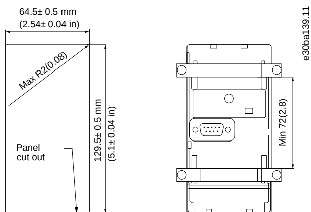
Illustration 27: Panel Mounting Kit Dimensions
