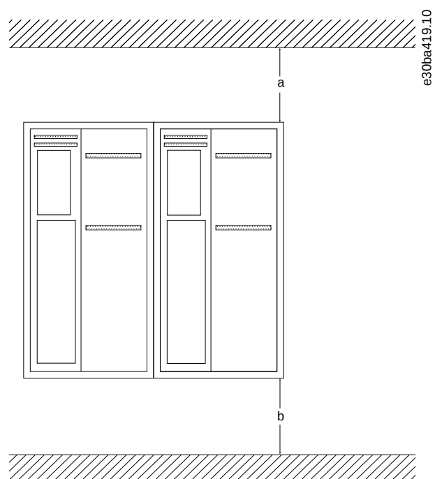
Illustration 33: Clearance
