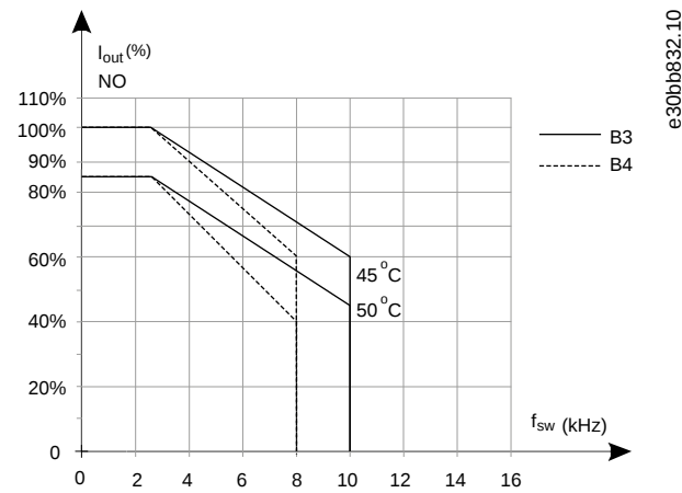
Illustration 47: Derating of I_{out} for Different T_{AMB,MAX} for Enclosure Sizes B3 and B4, using SFAVM
