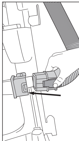
Attach hose. Align square end of hose with inlet and push in. Clip will snap to secure in place.
