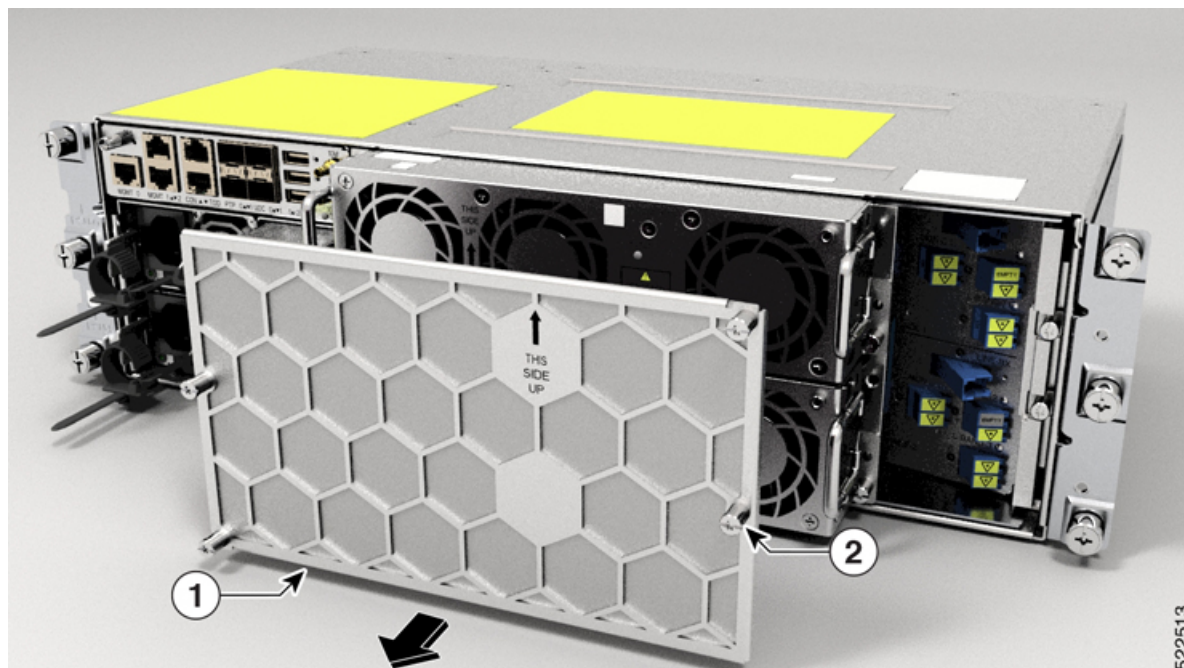
Figure 5: Removing the Fan Filter
