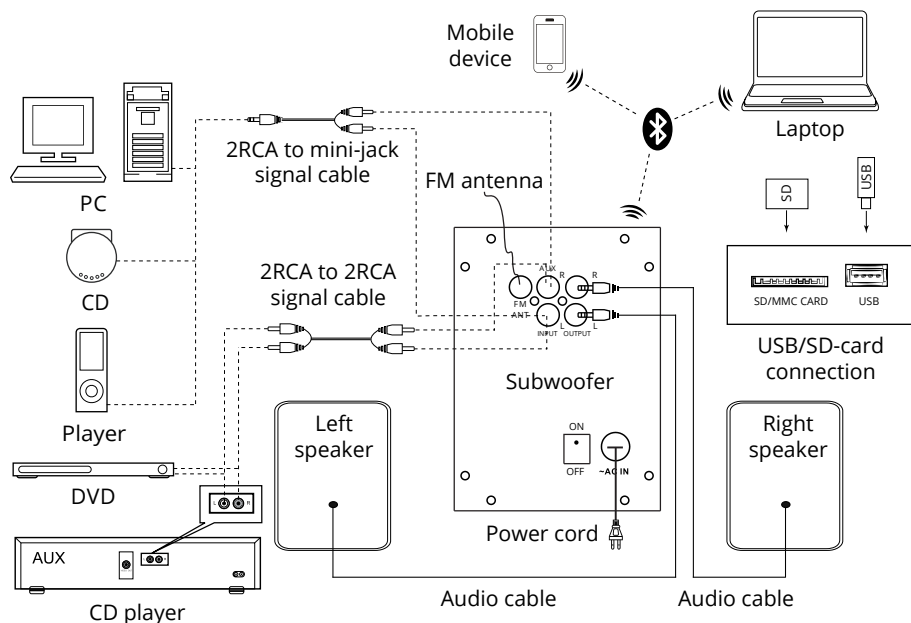
Fig. 4. Connection diagram
