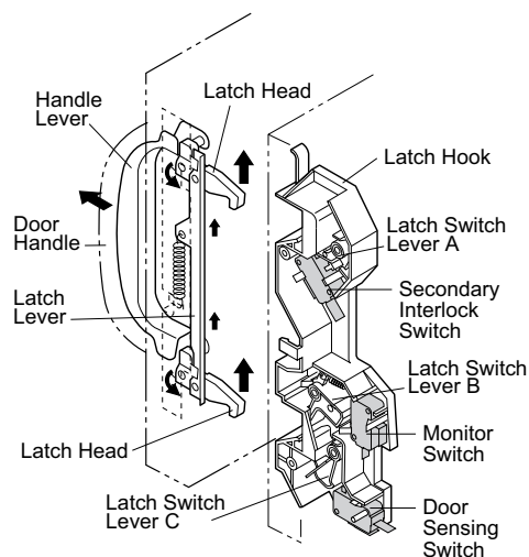
Figure C-5. Latch Switch Adjustments
