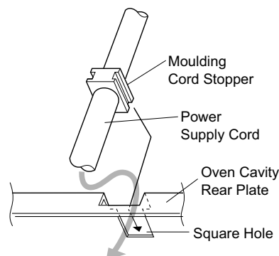
Figure C-3b. Power Supply Cord Replacement
