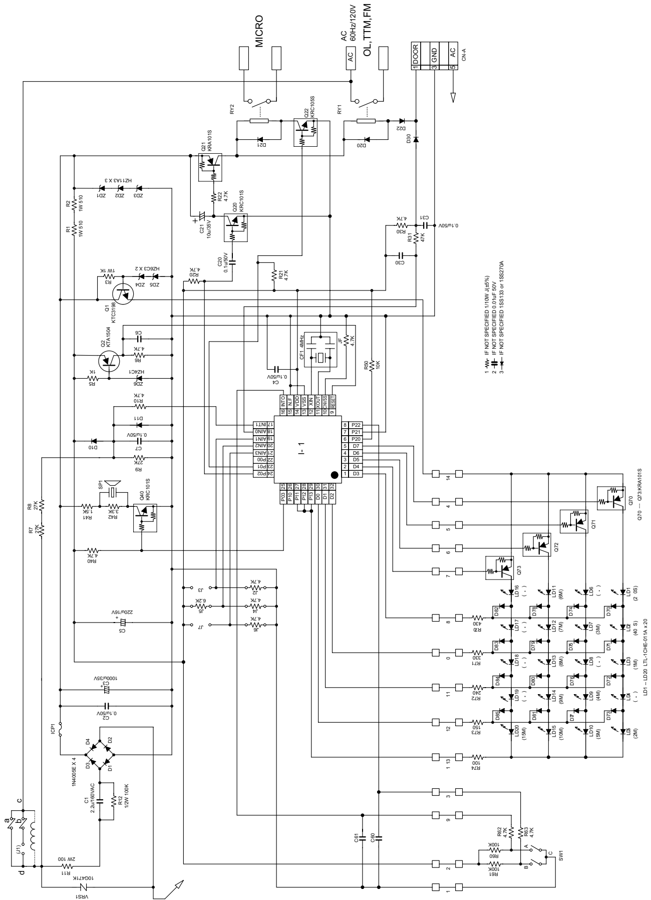
Figure S-2. Control Panel Circuit
