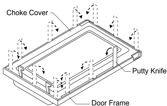
Figure C-6. Door Disassembly
