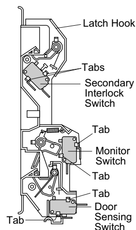
Figure C-4. Switches
