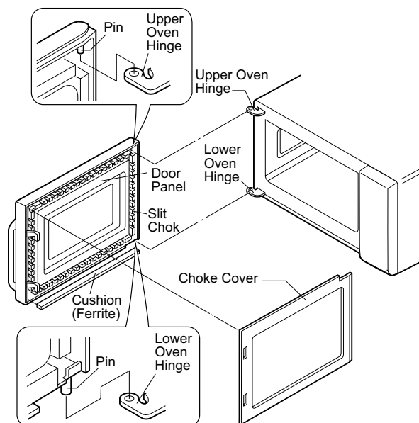
Figure C-7. Door Replacement
