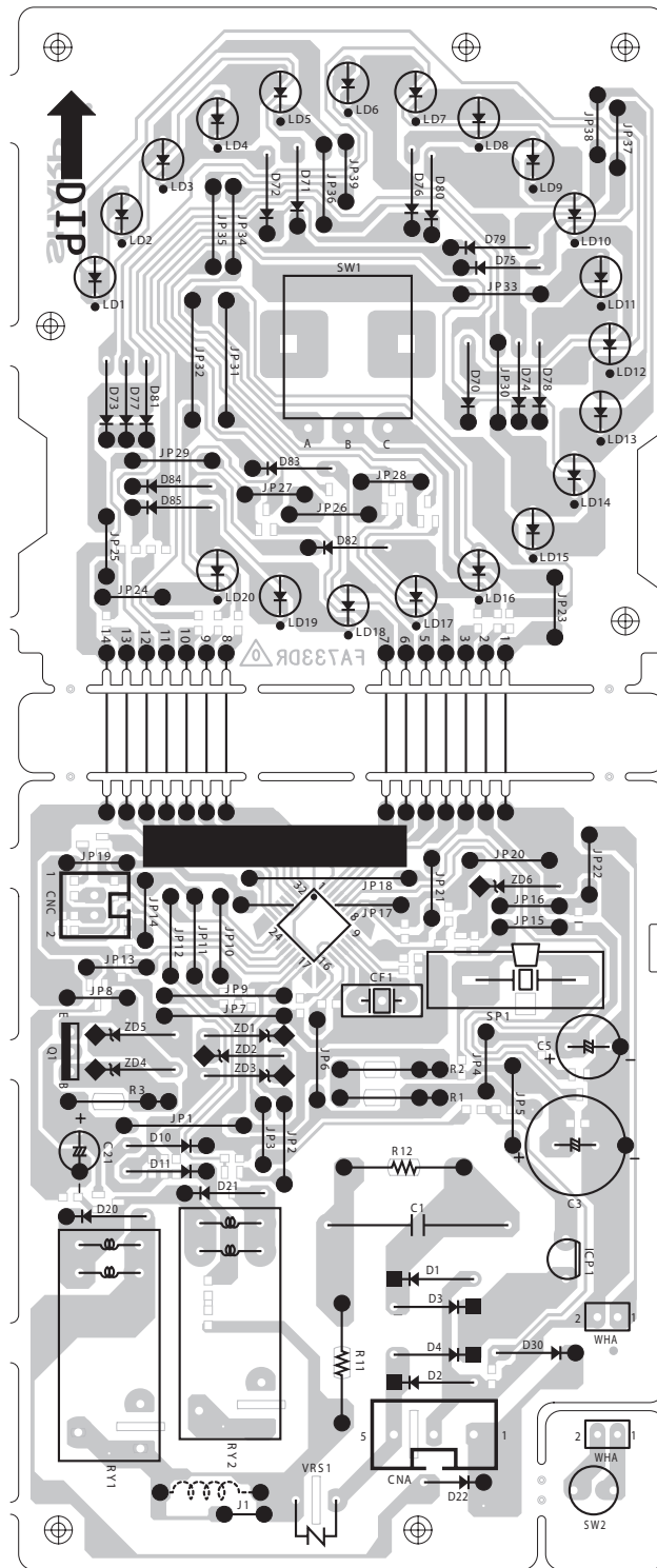
Figure S-3. Printed Wiring Board
