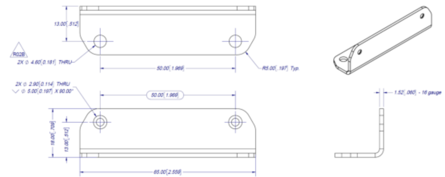
Figure 6: Bracket dimensions
