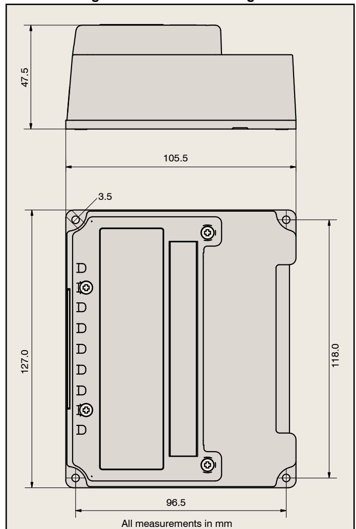
Figure 10 - Dimension Diagram
