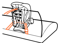
Lap belt with top tether
