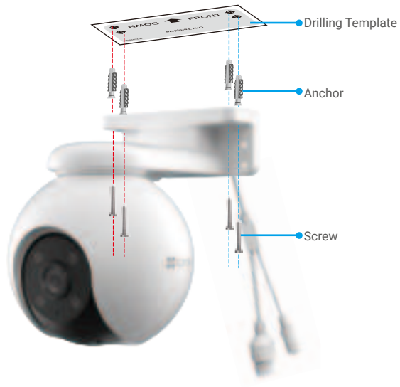
Fig. 1 Ceiling Mount
