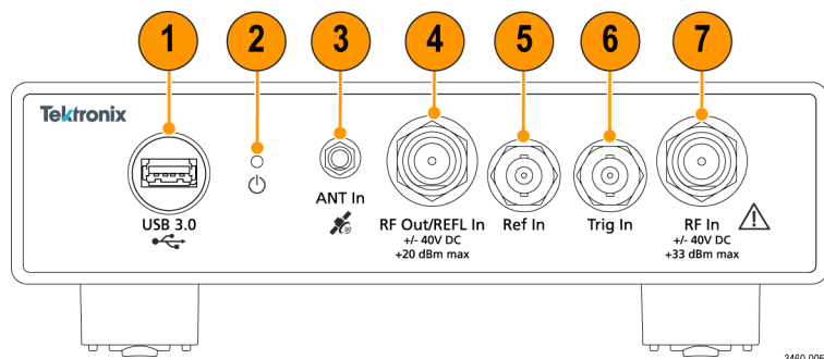
Figure 1: Front panel
