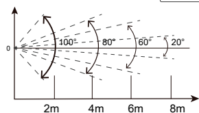
Diagram of PIR Detection Range
