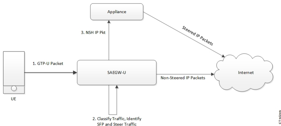
Figure 39: Uplink Packet Flow
