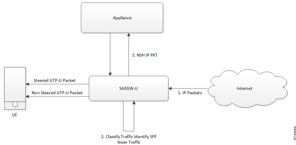
Figure 40: Downlink Packet Flow
