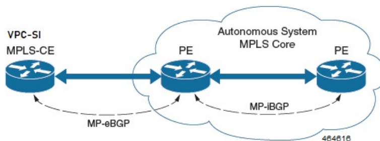
Figure 15: VPC-SI MPLS-CE to PE
