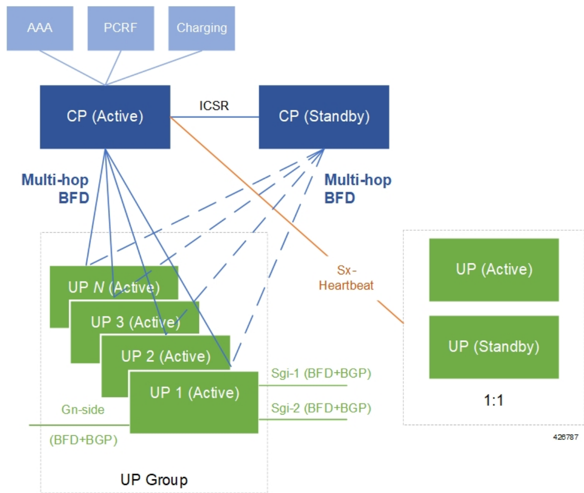
Figure 24: BFD Monitoring in N+2 Deployment
