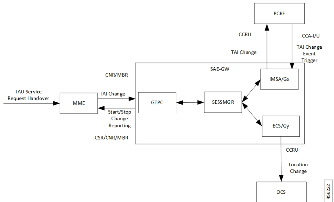
Figure 23: TAI Change Event Handling - Process Flow
